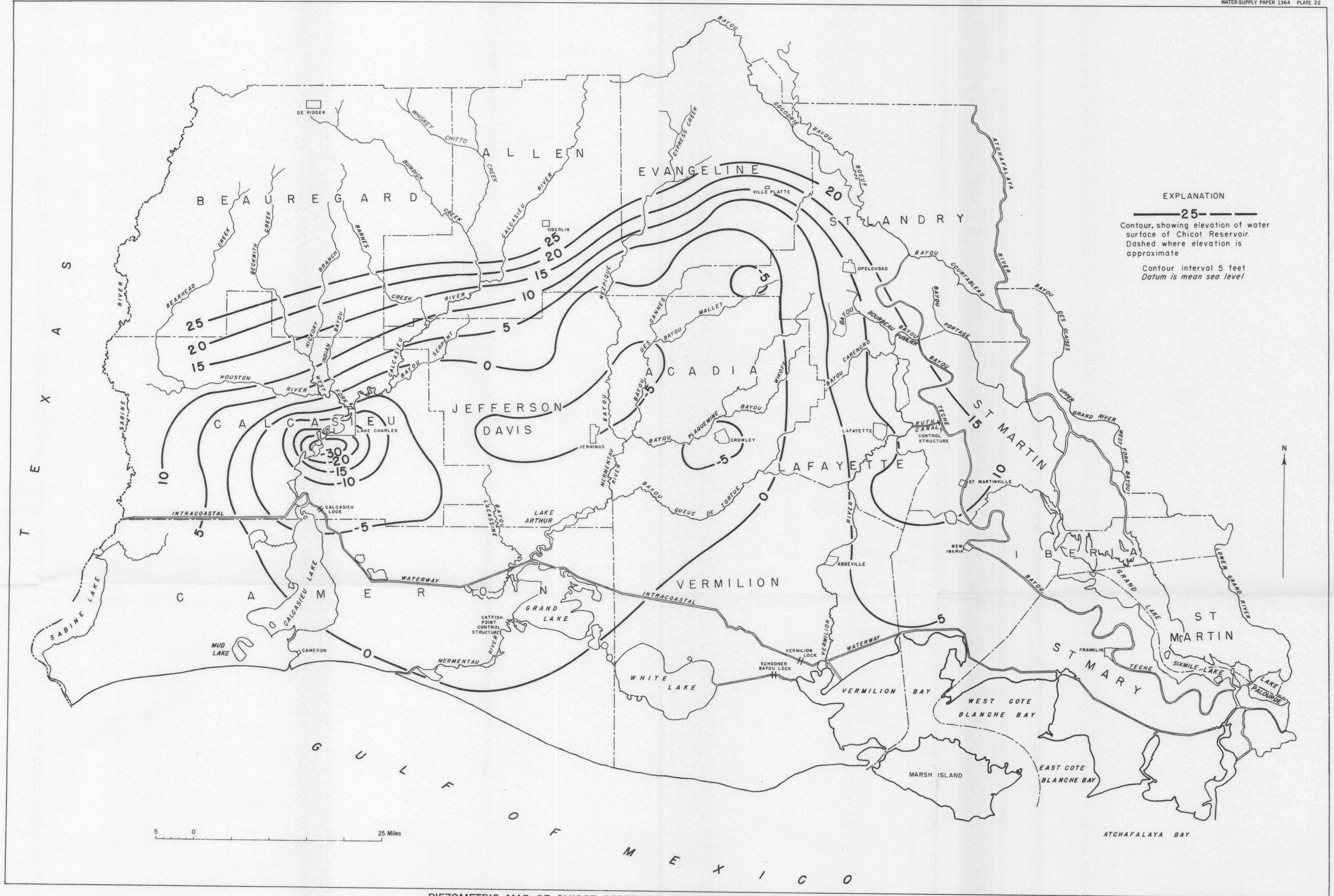
PIEZOMETRIC MAP OF CHICOT RESERVOIR, SOUTHWESTERN LOUISIANA, APRIL 1948
