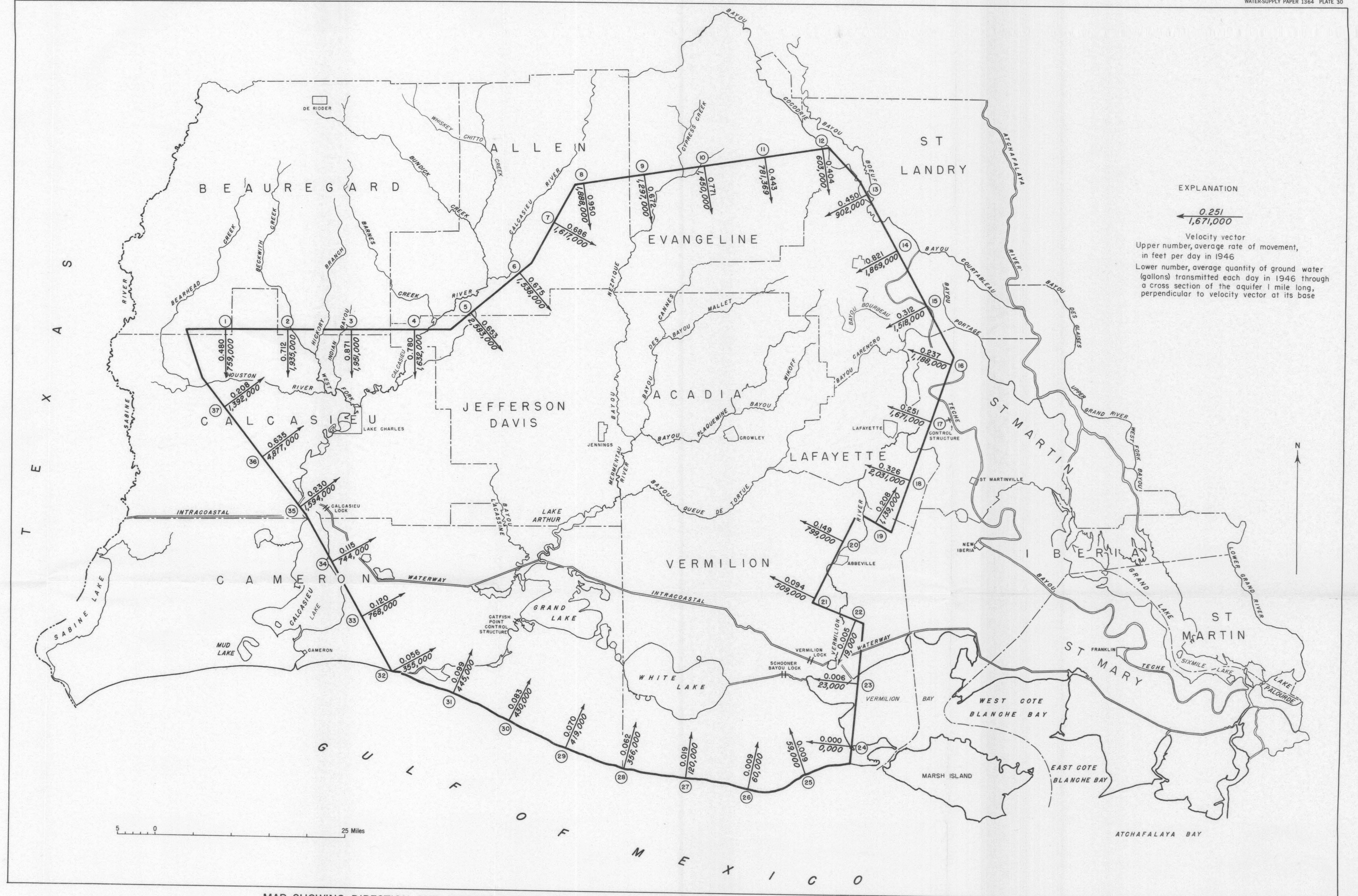
MAP SHOWING DIRECTION AND AVERAGE RATE OF GROUND-WATER MOVEMENT IN AREA OF HEAVY WITHDRAWAL, SOUTHWESTERN LOUISIANA, 1946
