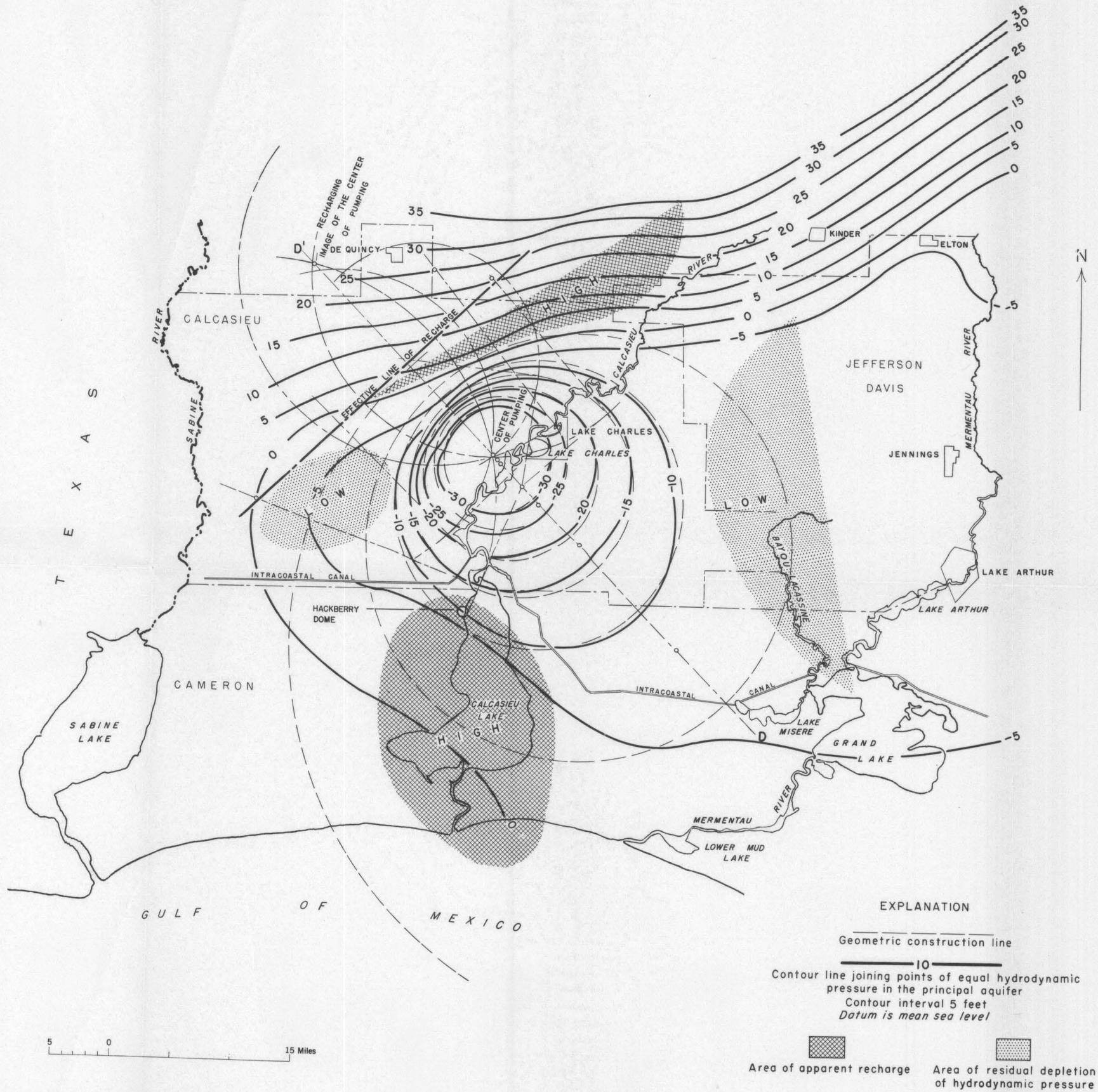
GEOMETRIC ANALYSIS OF PIEZOMETRIC CONDITIONS IN THE PRINCIPAL AQUIFER IN THE GREATER LAKE CHARLES AREA, SOUTHWESTERN LOUISIANA, MARCH 1951
