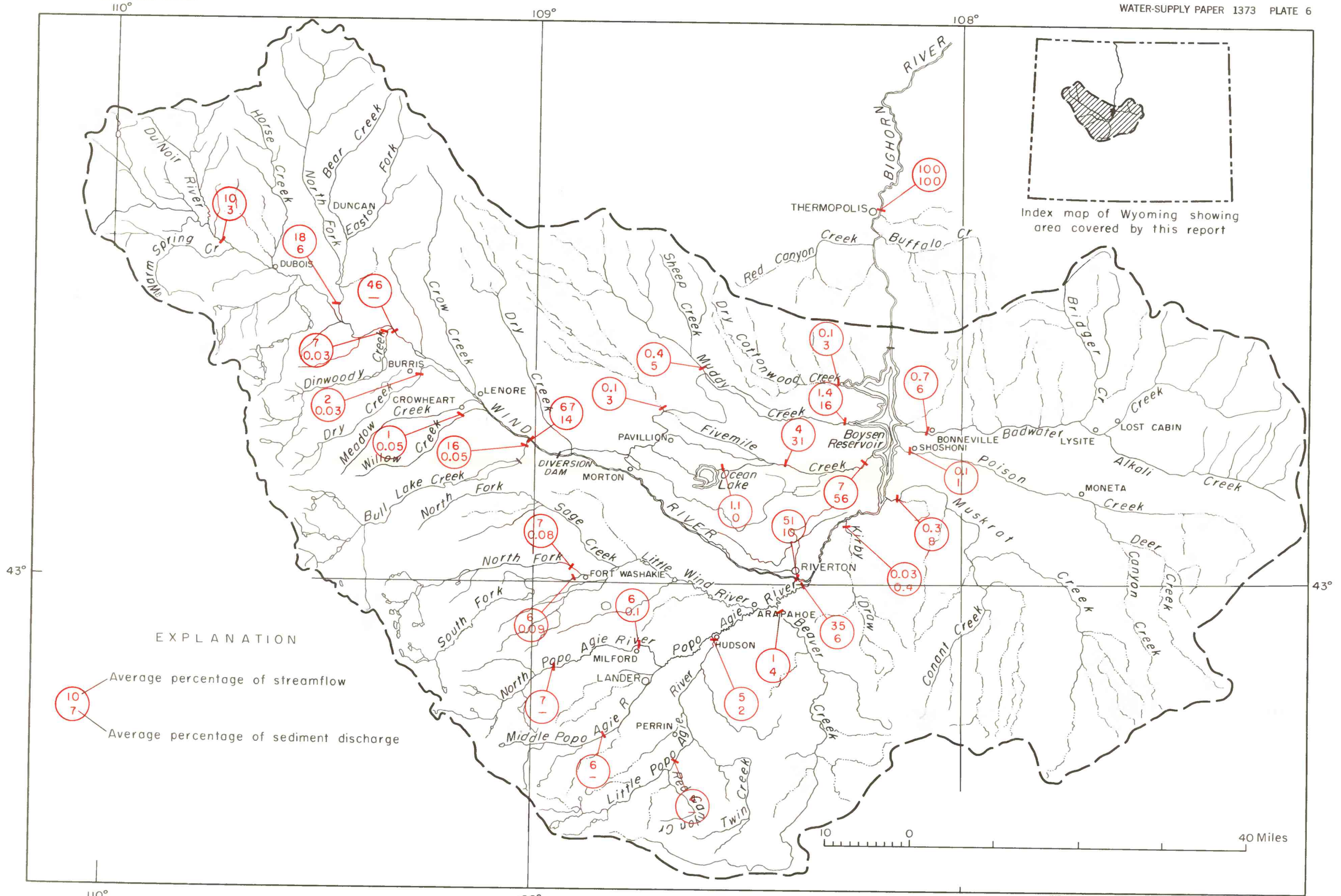
APPROXIMATE AVERAGE SEDIMENT DISCHARGE AND STREAMFLOW IN PERCENTAGE OF SEDIMENT DISCHARGE AND STREAMFLOW AT THERMOPOLIS, WYOMING
