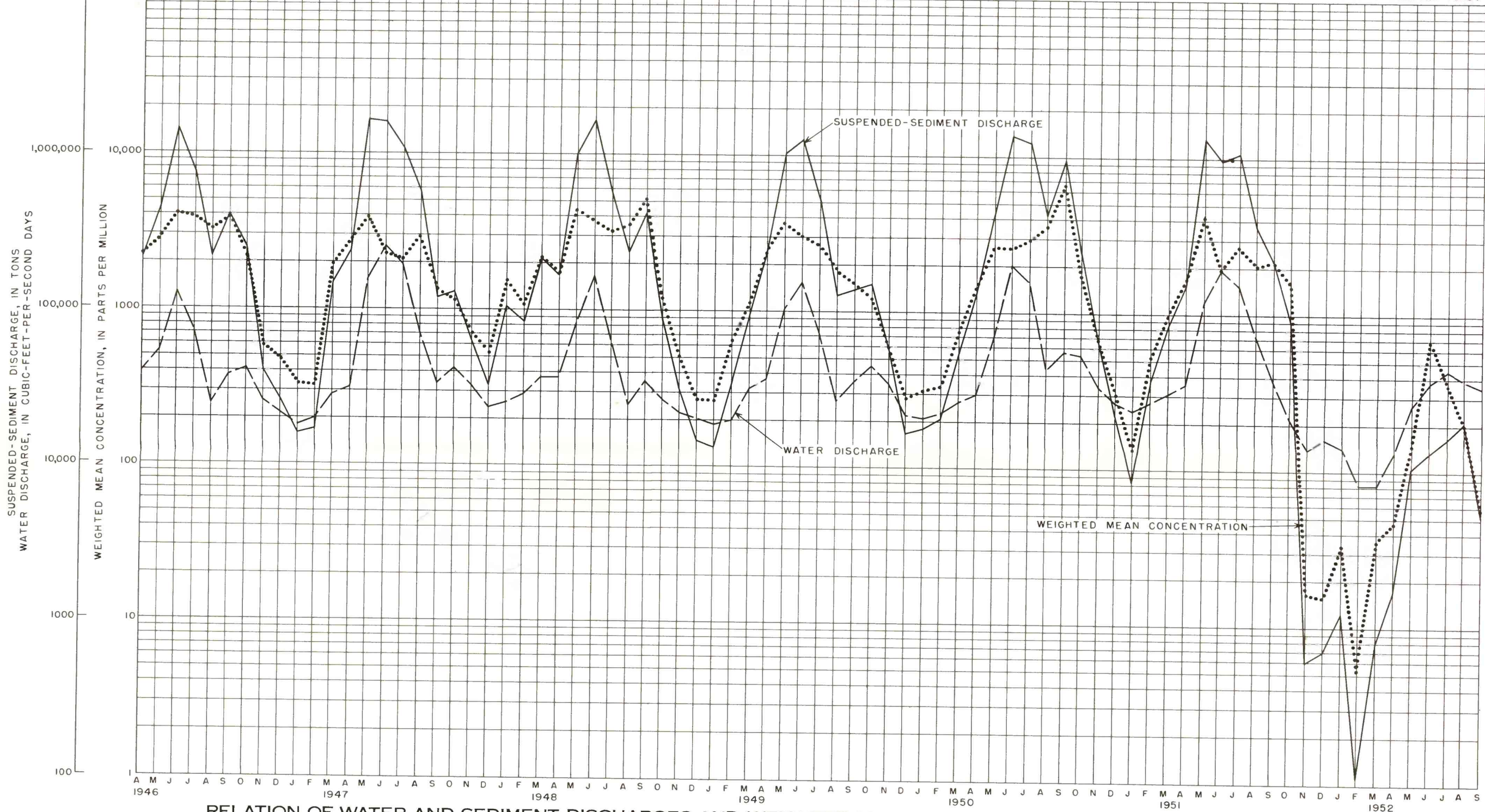
RELATION OF WATER AND SEDIMENT DISCHARGES AND WEIGHTED MEAN CONCENTRATION, BIG HORN RIVER AT THERMOPOLIS, OCTOBER 1, 1946, TO SEPTEMBER 30, 1952
