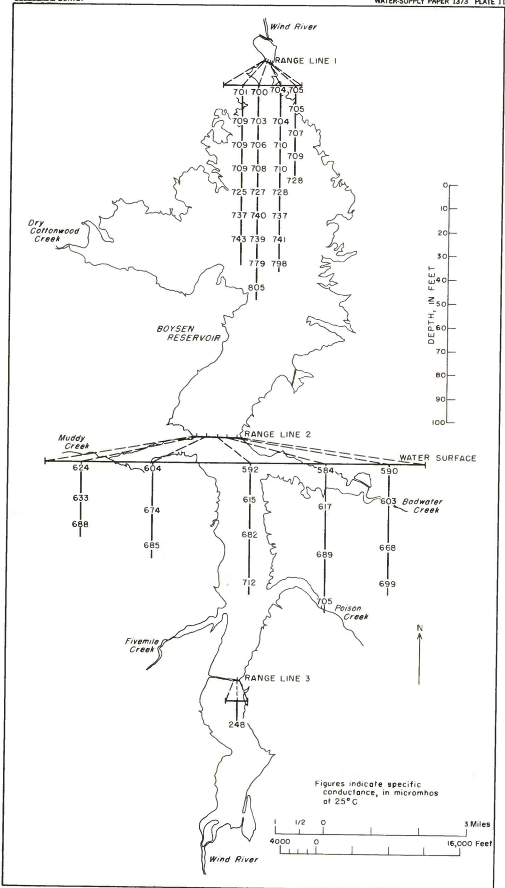
VERTICAL-AREAL MINERALIZATION IN BOYSEN RESERVOIR DURING PERIOD OF RAPID FILLING, JUNE 29, 1954
