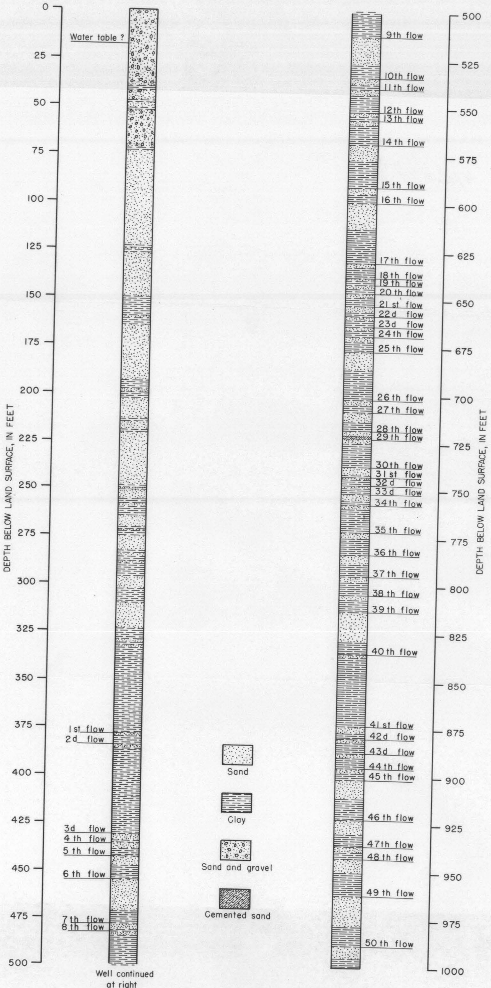
LOG OF WELL ON BACA GRANT
