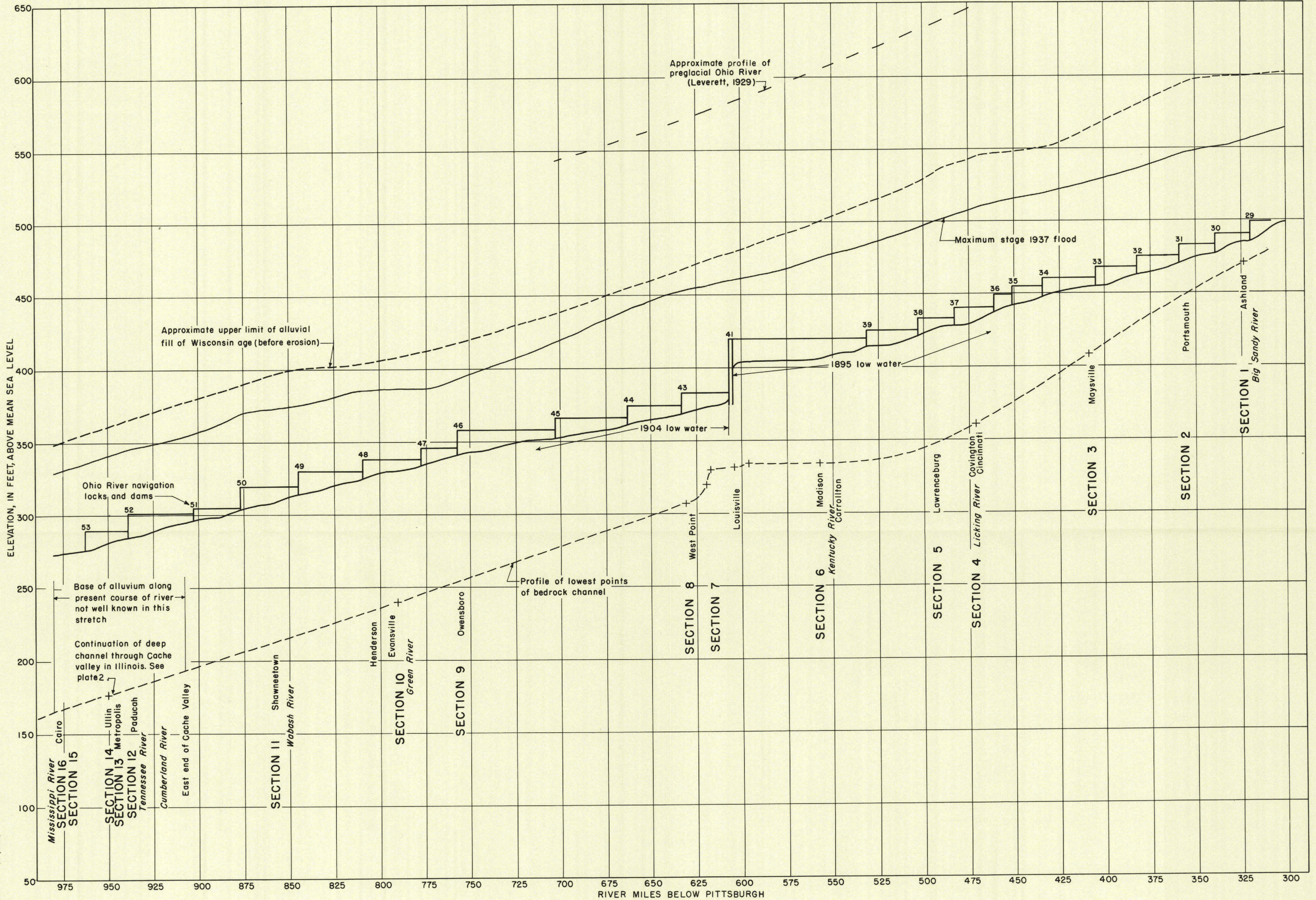
PROFILES OF THE OHIO RIVER FROM WEST VIRGINIA TO THE MISSISSIPPI RIVER SHOWING ELEVATIONS OF THE BEDROCK CHANNEL, POOL LEVELS, AND FORMER RIVER LEVELS
