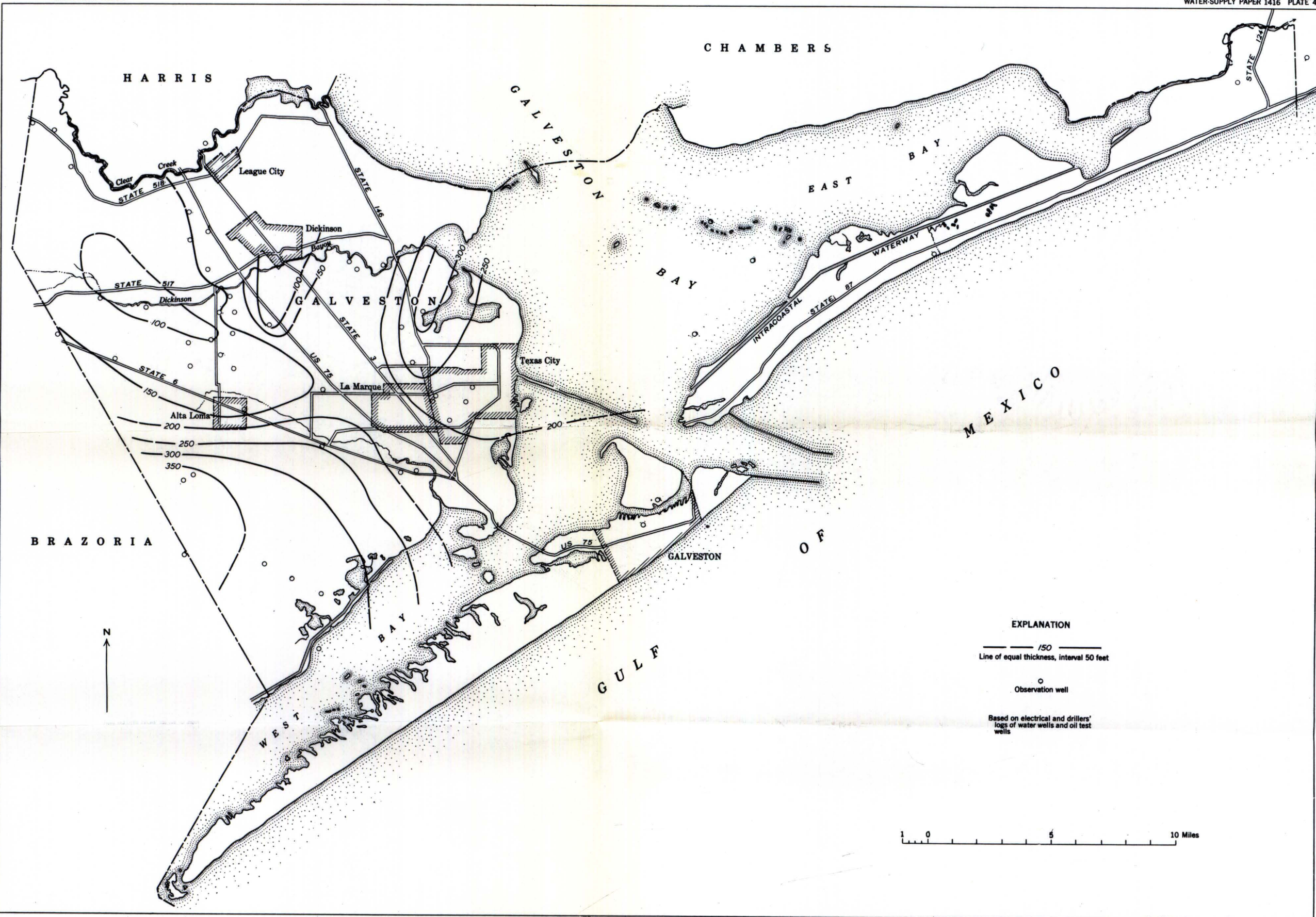
ISOPACH MAP OF THE "ALTA LOMA" SAND IN GALVESTON COUNTY, TEXAS
