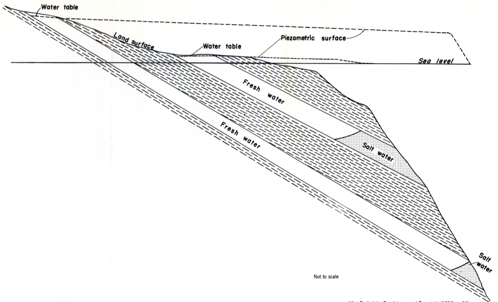
THEORETICAL RELATION BETWEEN FRESH WATER AND SALT WATER IN WATER-BEARING SANDS WHEN NOT DISTURBED BY PUMPING
