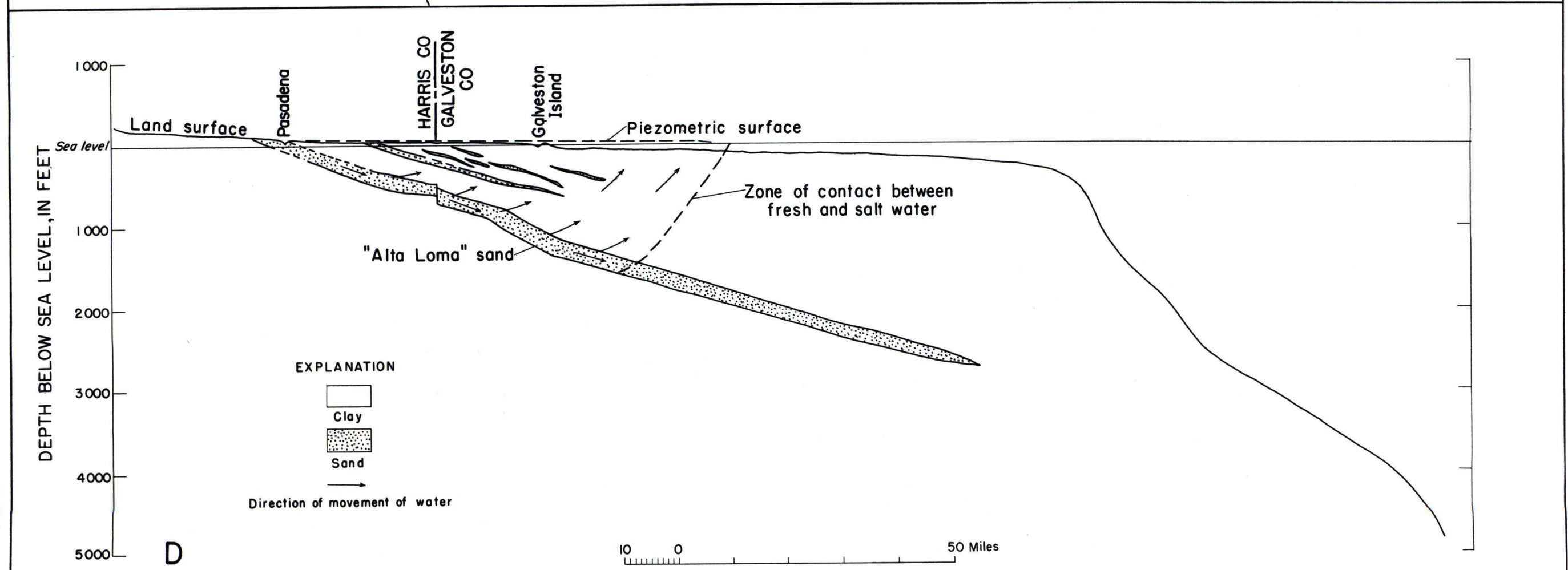
DIAGRAMS SHOWING POSSIBLE METHODS BY WHICH THE COASTAL AQUIFERS WERE FLUSHED
