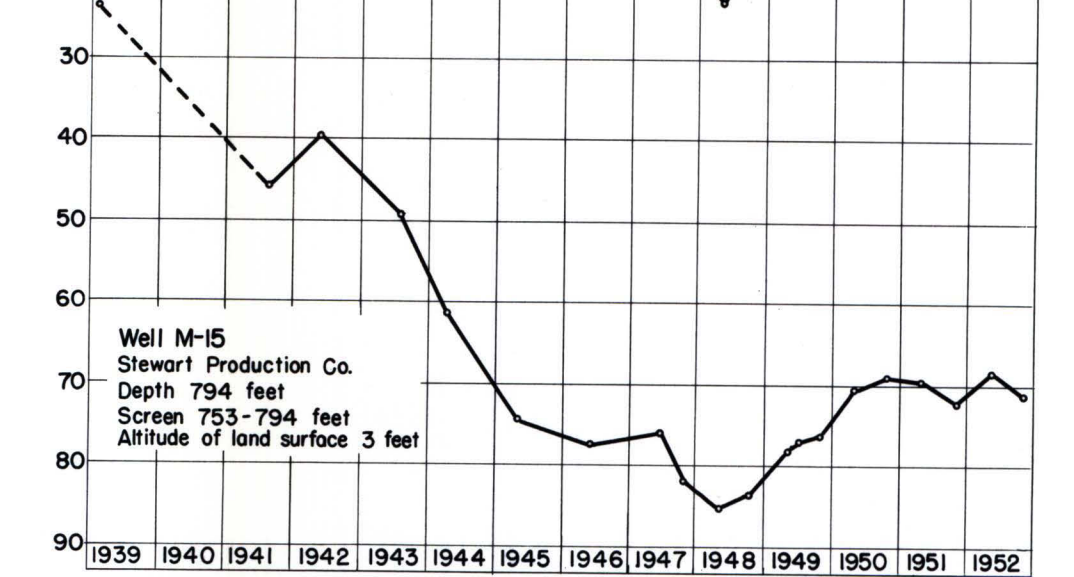
GRAPHS SHOWING THE FLUCTUATIONS OF ARTESIAN PRESSURE IN 10 WELLS IN THE "ALTA LOMA" SAND, GALVESTON COUNTY, TEXAS
