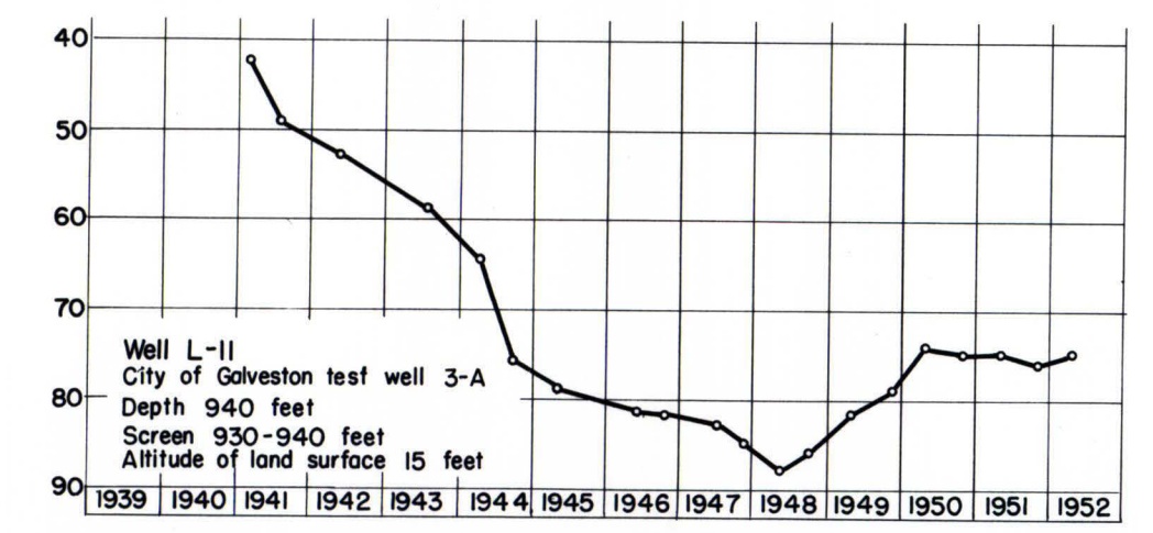
GRAPHS SHOWING THE FLUCTUATIONS OF ARTESIAN PRESSURE IN 10 WELLS IN THE "ALTA LOMA" SAND, GALVESTON COUNTY, TEXAS
