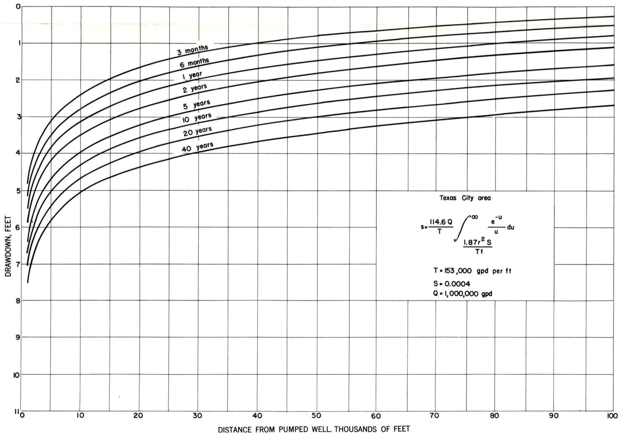
THEORETICAL DRAWDOWN IN AN INFINITE AQUIFER, COMPUTED ACCORDING TO THE NONEQUILIBRIUM FORMULA
