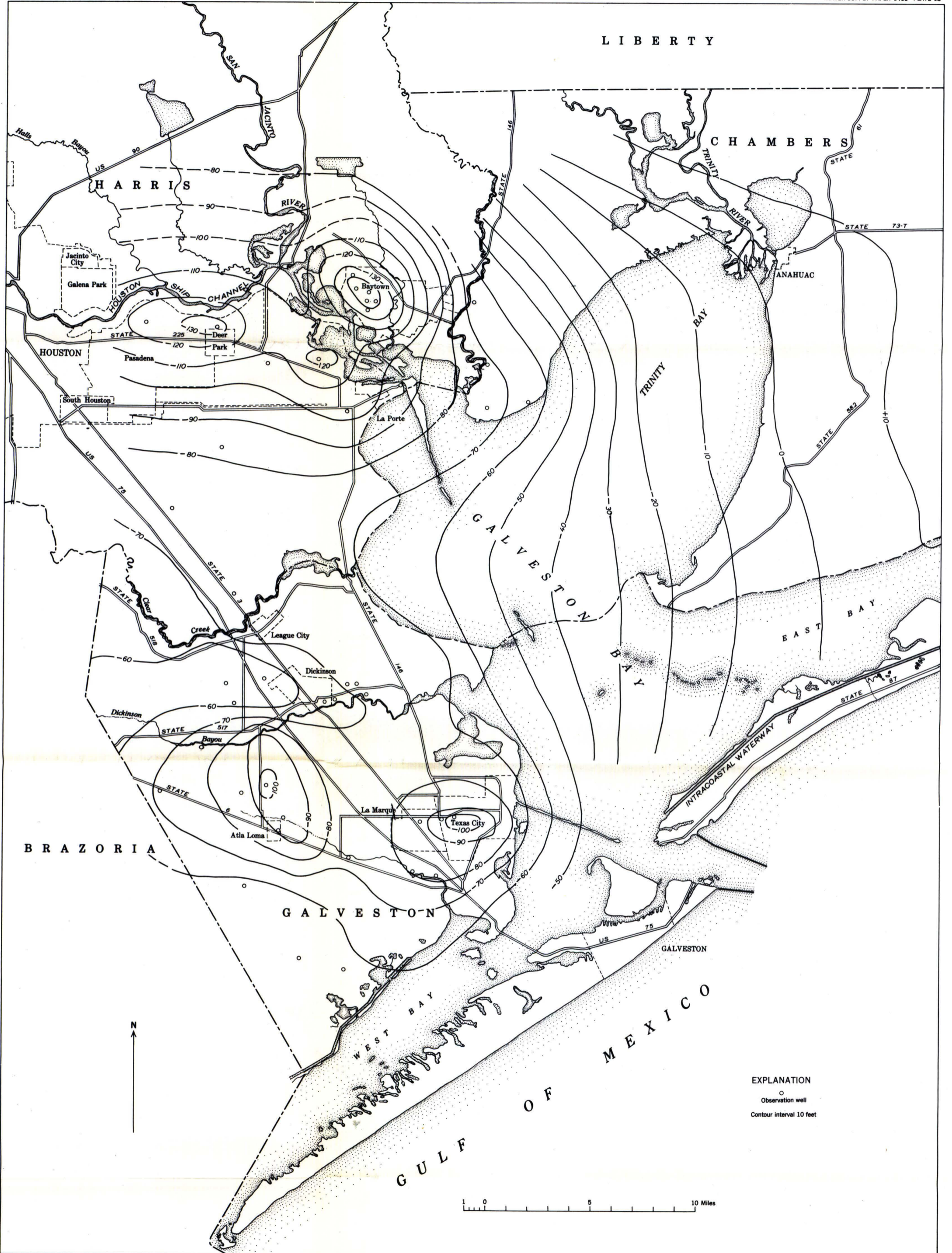
APPROXIMATE WATER LEVEL, IN FEET, ABOVE OR BELOW MEAN SEA LEVEL, IN WELLS SCREENED IN THE "ALTA LOMA" SAND IN GALVESTON, HARRIS, AND CHAMBERS COUNTIES, TEXAS, MAY 1948
