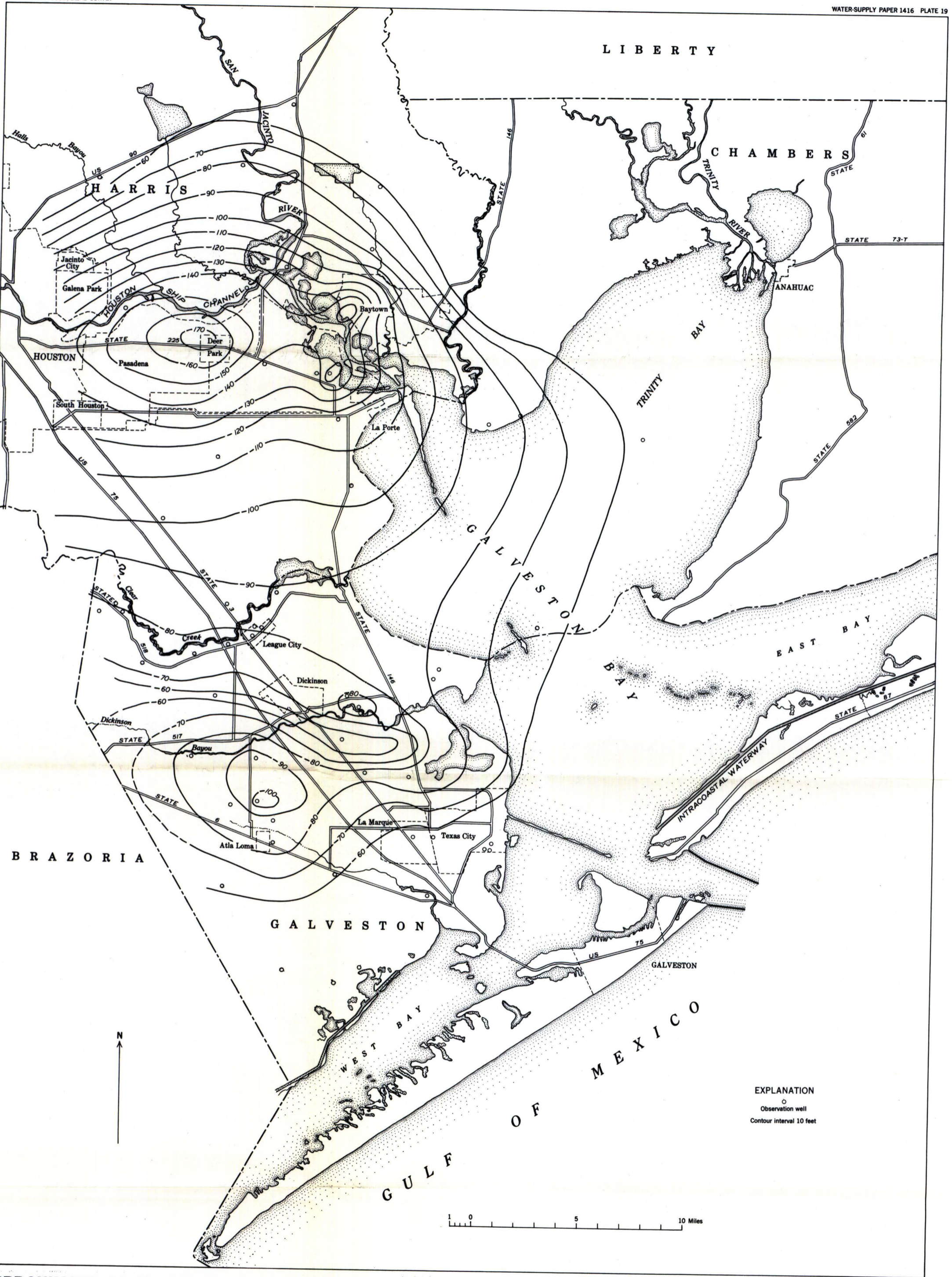
APPROXIMATE DEPTH BELOW MEAN SEA LEVEL, IN FEET, IN WELLS SCREENED IN THE "ALTA LOMA" SAND IN GALVESTON, HARRIS, AND CHAMBERS COUNTIES, TEXAS, MAY 1952
