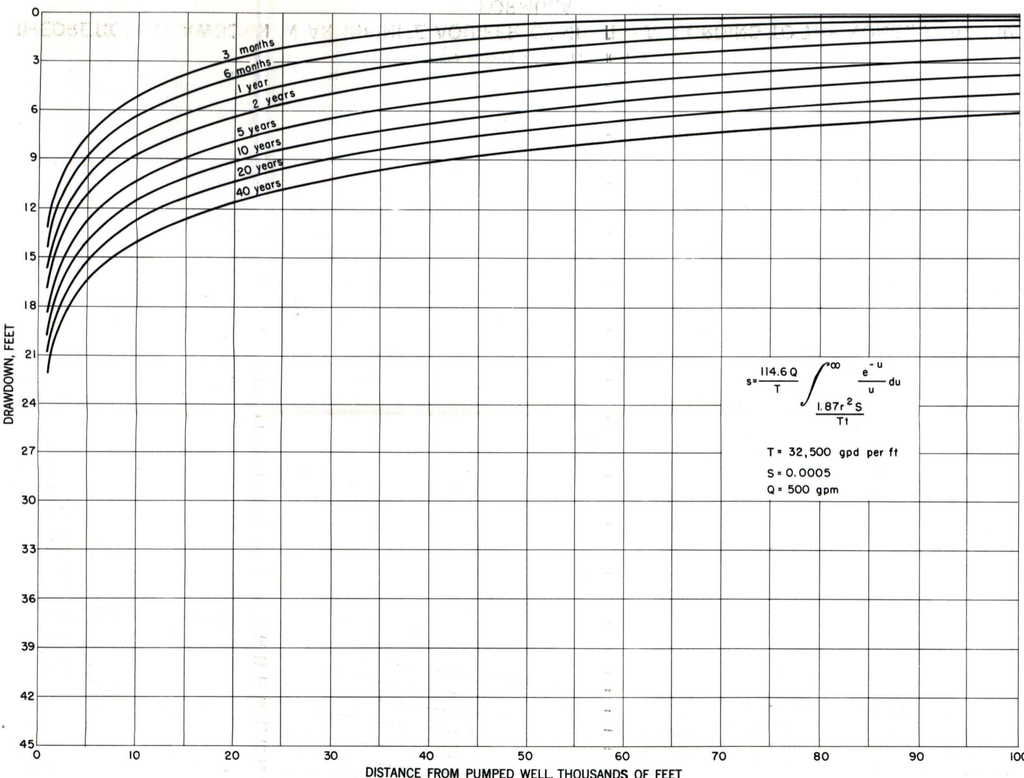
THEORETICAL DRAWDOWN IN AN INFINITE AQUIFER, COMPUTED ACCORDING TO THE NONEQUILIBRIUM FORMULA
