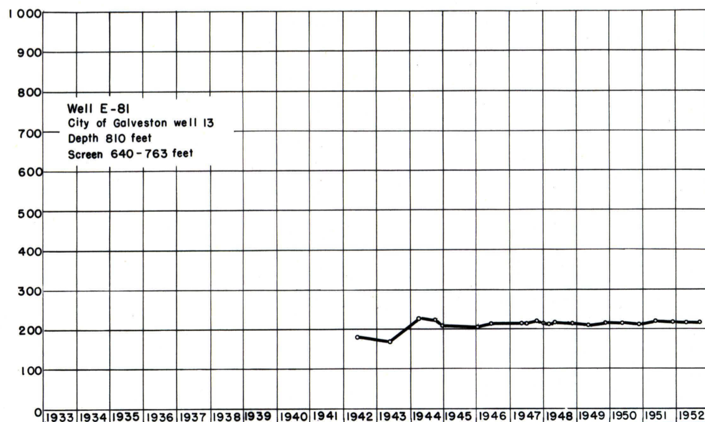
419189 O-57 (In pocket) GRAPHS SHOWING FLUCTUATION OF CHLORIDE CONTENT OF THE WATER FROM WELLS IN THE "ALTA LOMA" SAND NORTH OF ALTA LOMA, GALVESTON AND HARRIS COUNTIES, TEXAS
