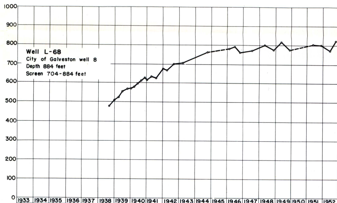
GRAPHS SHOWING FLUCTUATION OF CHLORIDE CONTENT OF THE WATER FROM WELLS IN THE "ALTA LOMA" SAND IN THE VICINITY OF ALTA LOMA, GALVESTON COUNTY, TEXAS
