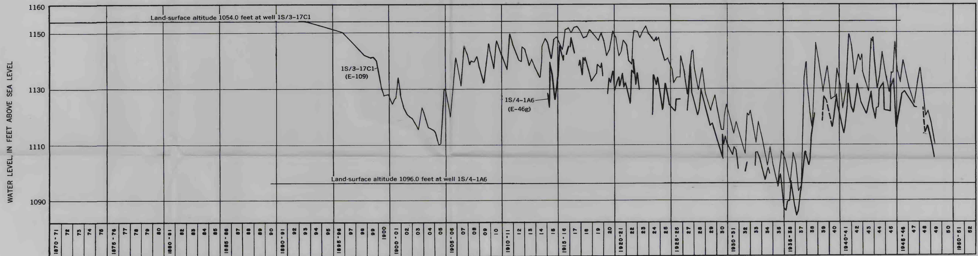
CUMULATIVE-DEPARTURE GRAPH OF PRECIPITATION, AND LONG-TERM HYDROGRAPHS OF SELECTED WELLS IN SAN BERNARDINO AREA, CALIFORNIA
