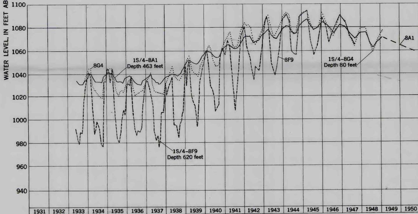
HYDROGRAPHS OF WELLS IN BUNKER HILL BASIN NEAR COLTON, CALIFORNIA
