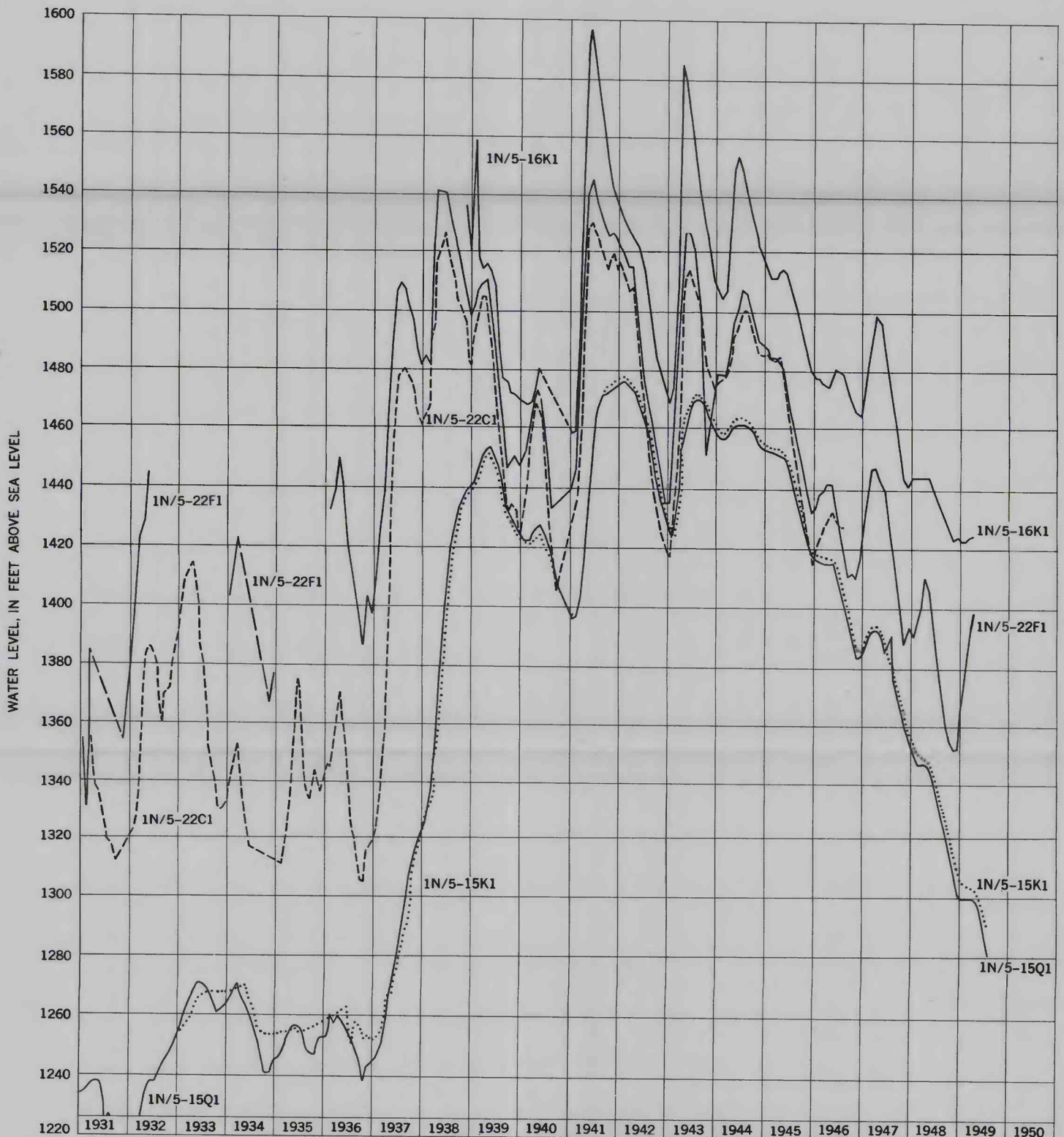
HYDROGRAPHS OF SELECTED WELLS ALONG LYTLE CREEK, CALIFORNIA
