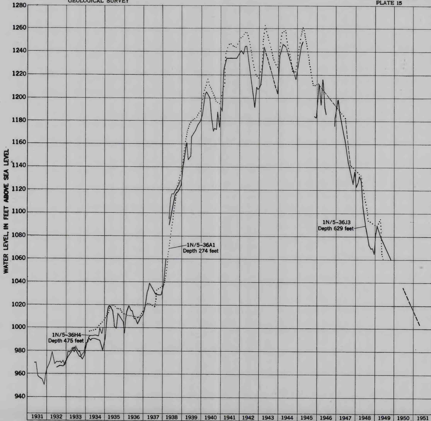
HYDROGRAPHS OF SELECTED WELLS IN LOWER LYTLE BASIN, CALIFORNIA
