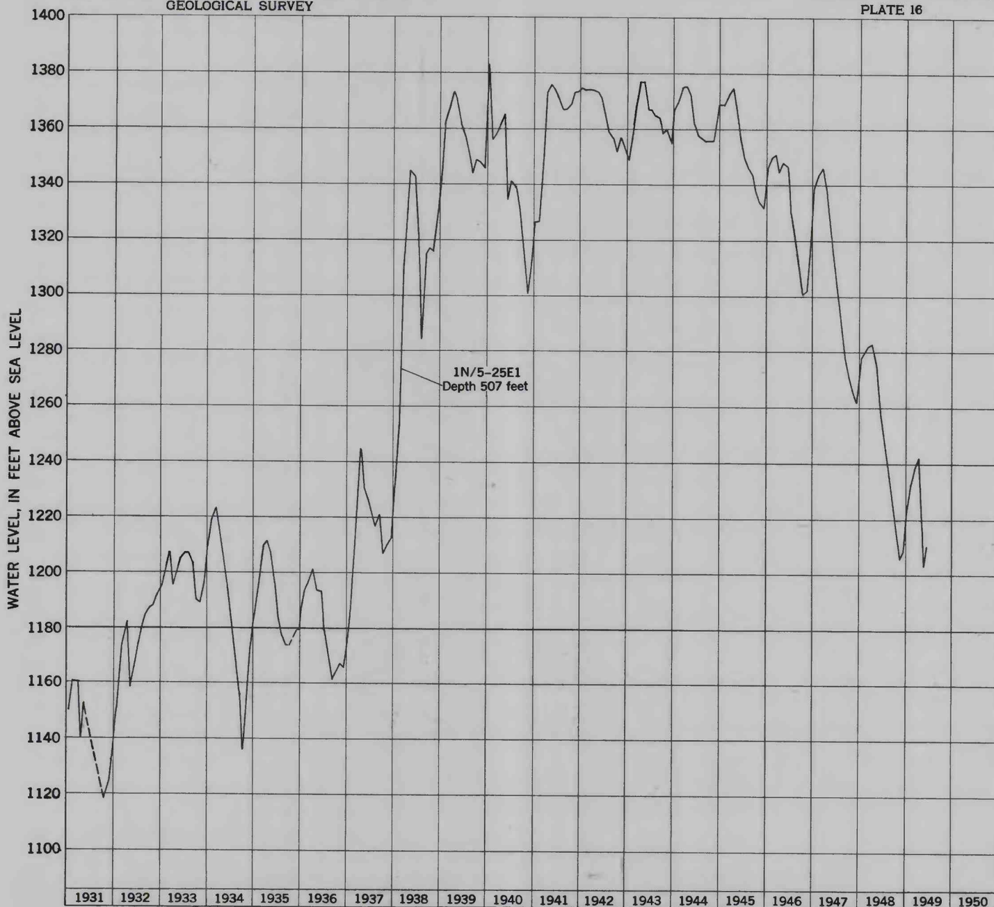
HYDROGRAPH OF A WELL IN UPPER LYTLE BASIN, CALIFORNIA
