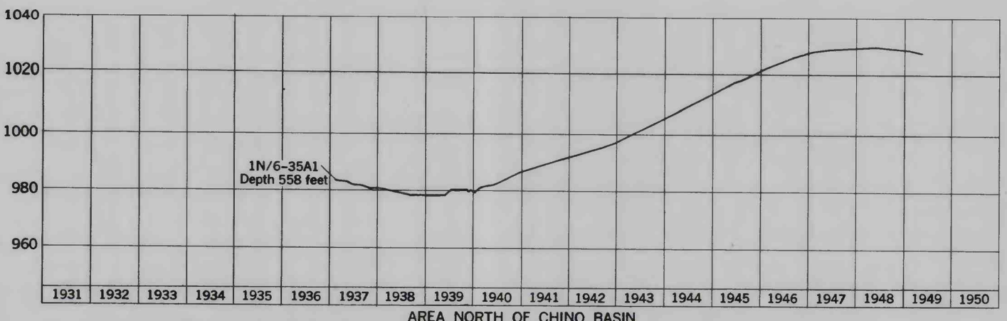
HYDROGRAPHS OF WELLS IN AREAS OF THE RIALTO-COLTON AND CHINO BASINS, AND AREA NORTH OF CHINO BASIN, CALIFORNIA
