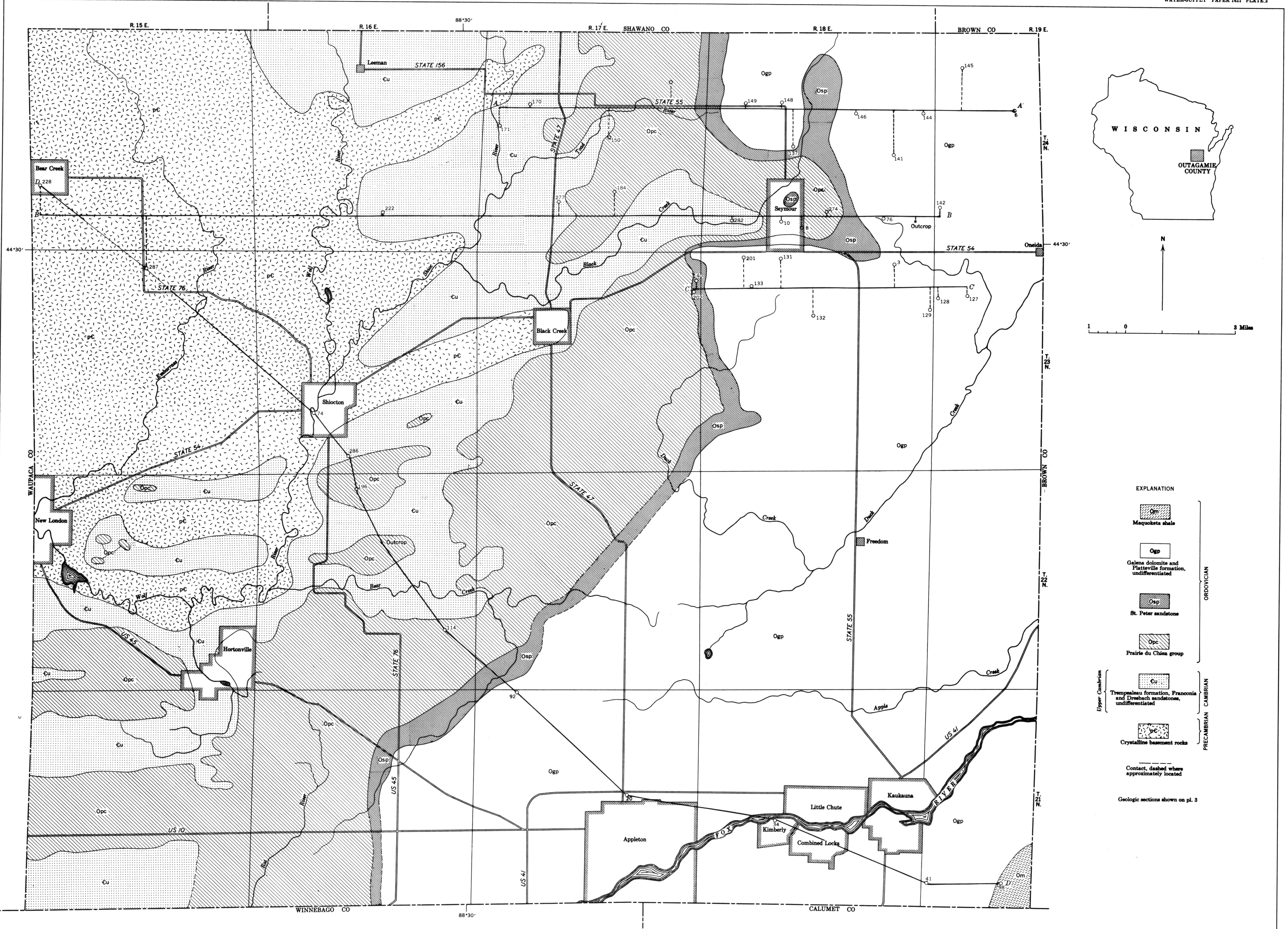
MAP OF OUTAGAMIE COUNTY, WISCONSIN, SHOWING BEDROCK GEOLOGY
