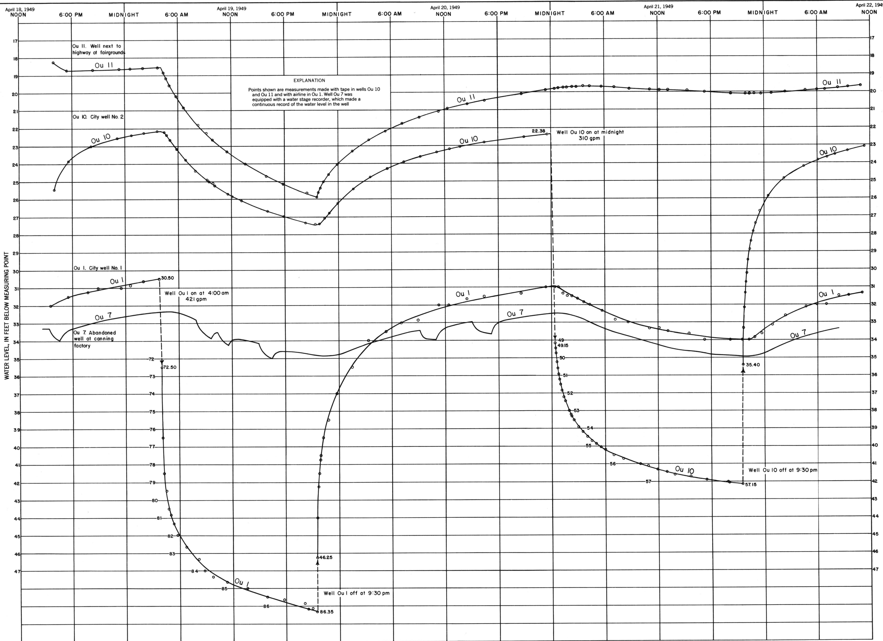
HYDROGRAPHS OF WELLS AT SEYMOUR, WISCONSIN, DURING PUMPING TESTS
