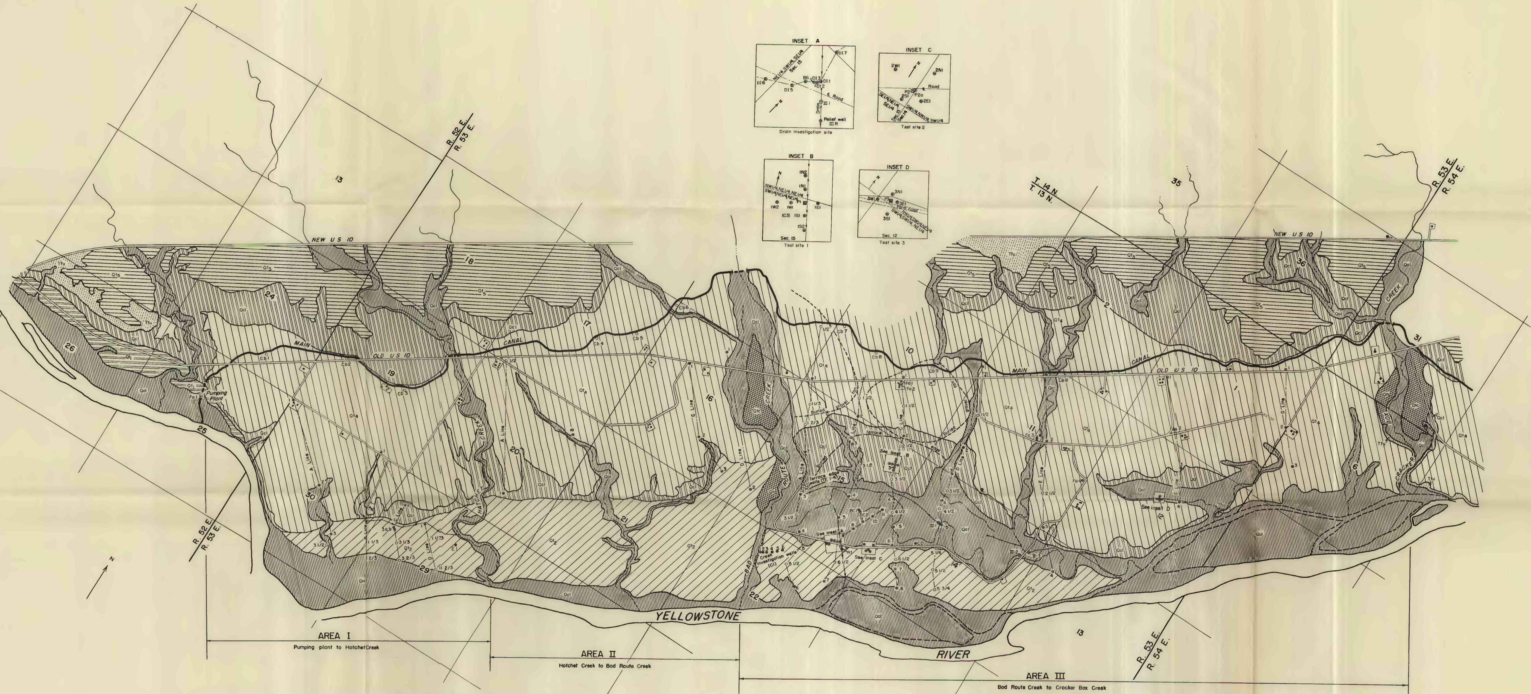
GEOLOGIC MAP OF AREAS I, II, AND III, FIRST DIVISION, BUFFALO RAPIDS IRRIGATION PROJECT, MONTANA, SHOWING LOCATION OF WELLS, TEST HOLES, AND SPRINGS
