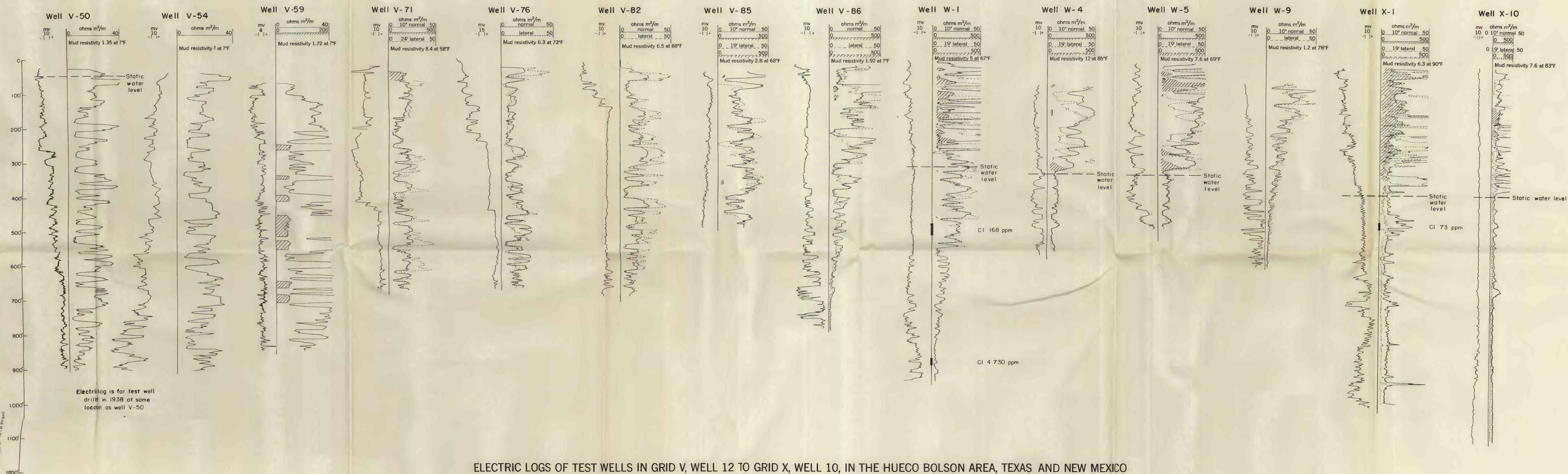
ELECTRIC LOGS OF TEST WELLS IN GRID V, WELL 12 TO GRID X, WELL 10, IN THE HUECO BOLSON AREA, TEXAS AND NEW MEXICO
