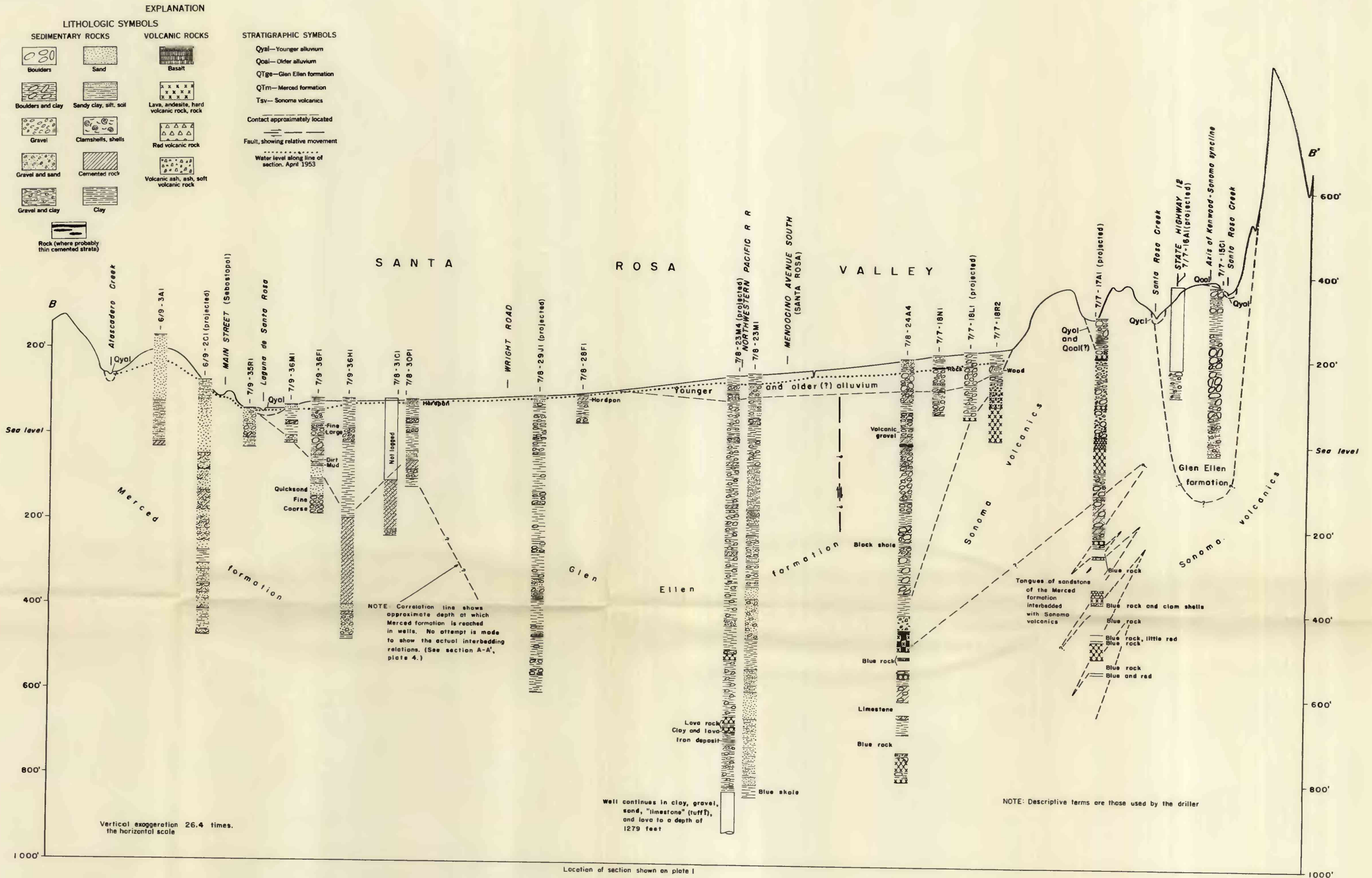
GEOLOGIC SECTION ACROSS THE MIDDLE OF SANTA ROSA VALLEY, CALIFORNIA, SHOWING STRATIGRAPHIC RELATIONS AND LITHOLOGY
