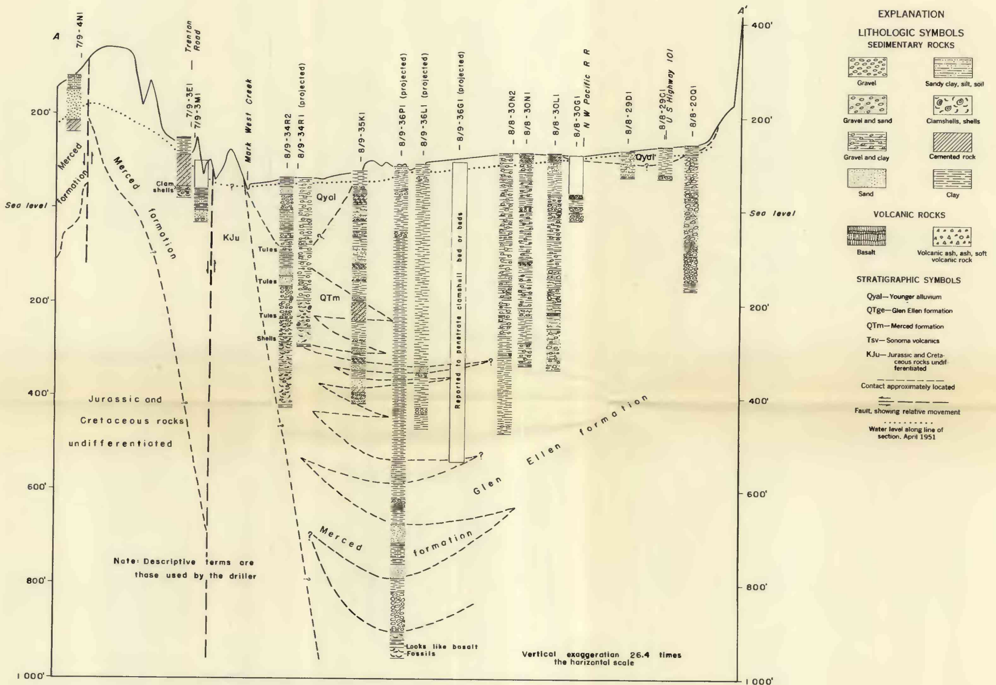
GEOLOGIC SECTION ACROSS THE NORTH END OF SANTA ROSA VALLEY, CALIFORNIA, SHOWING STRATIGRAPHIC RELATIONS AND LITHOLOGY
