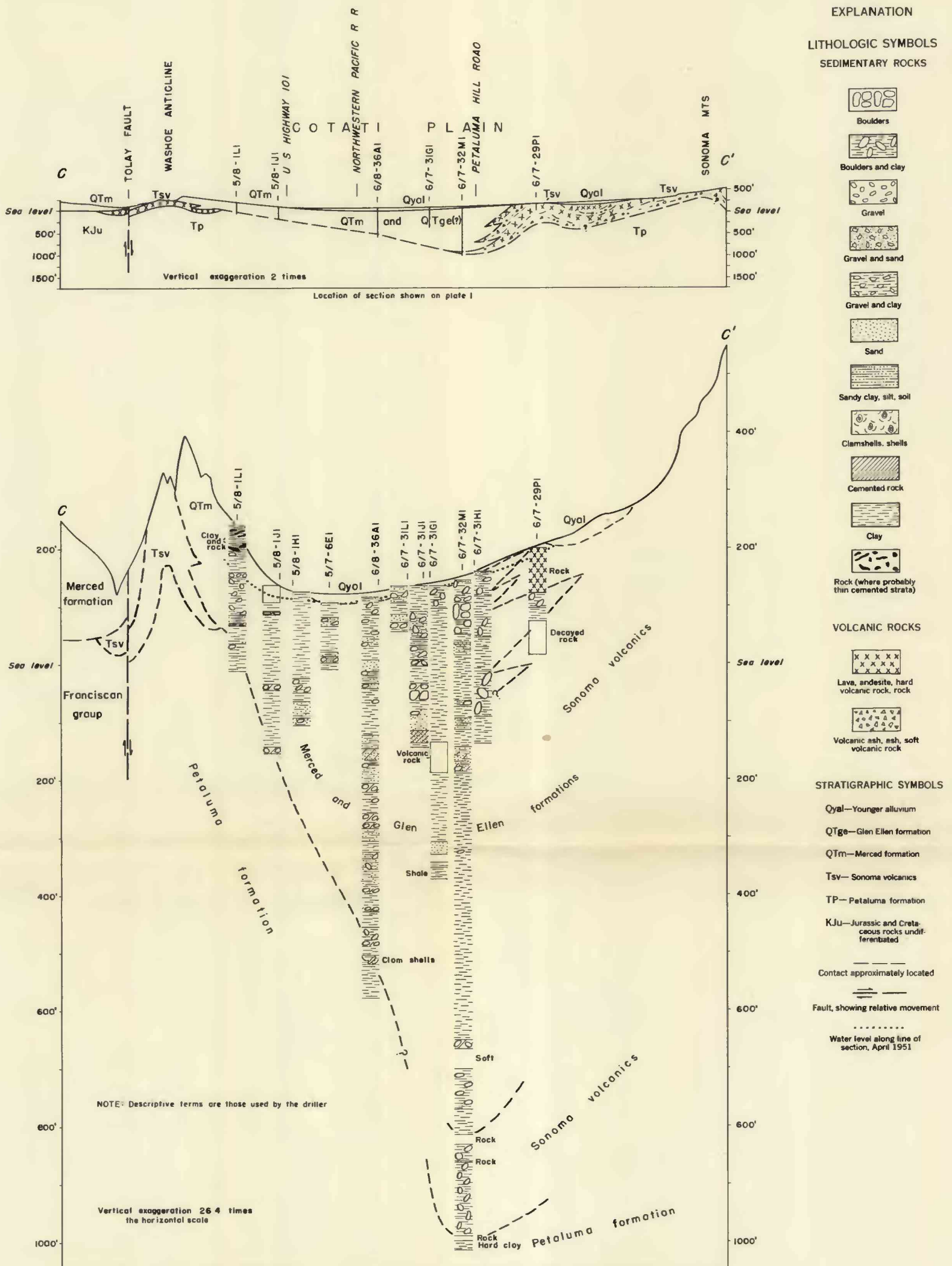
GEOLOGIC SECTION ACROSS SOUTHERN PART OF COTATI PLAIN, CALIFORNIA, SHOWING STRATIGRAPHIC RELATIONS AND LITHOLOGY
