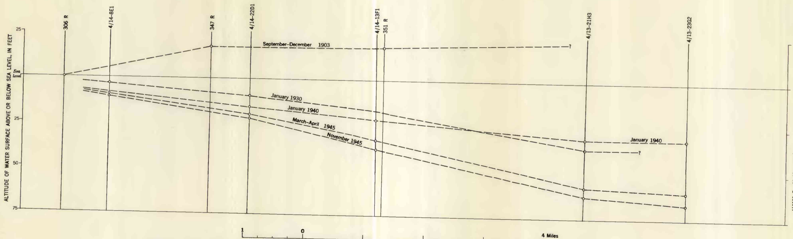
GEOLOGIC SECTION F-F', FROM REDONDO BEACH TO LONG BEACH, CALIFORNIA; ALSO WATER-LEVEL PROFILES OF 1903-45
