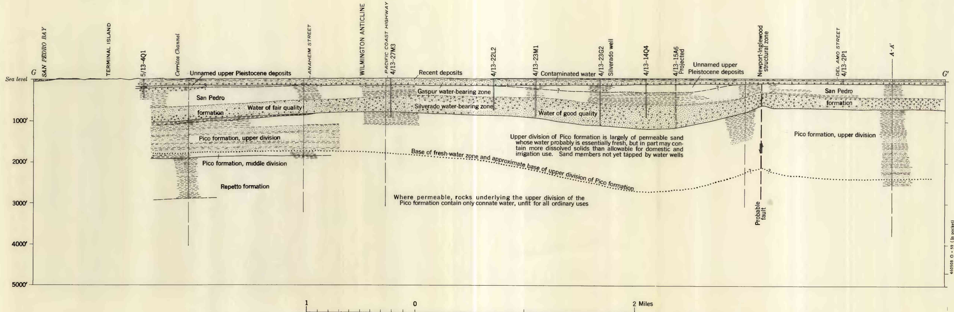
GEOLOGIC SECTION G-G', FROM TERMINAL ISLAND THROUGH DOMINGUEZ GAP, CALIFORNIA
