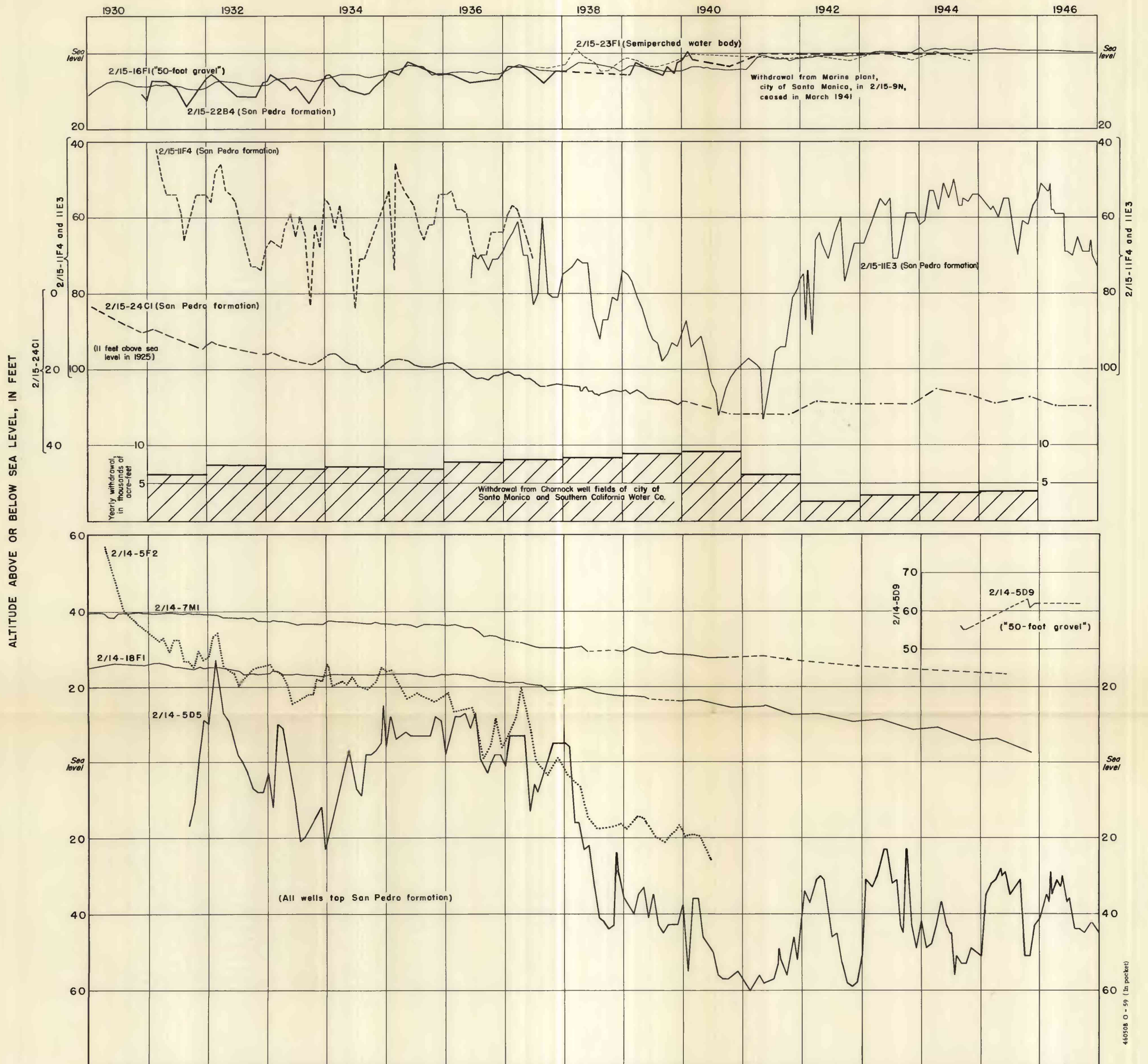
HYDROGRAPHS FOR SELECTED WELLS IN BALLONA GAP, CALIFORNIA
