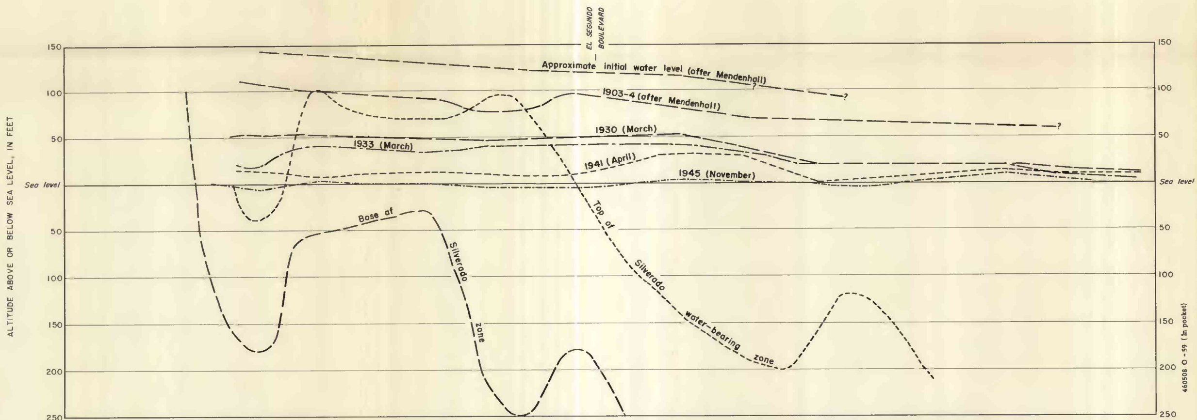
SECTION ALONG THE CREST OF THE NEWPORT-INGLEWOOD UPLIFT FROM BALDWIN HILLS TO LONG BEACH, CALIFORNIA, SHOWING THE GENERALIZED POSITION OF WATER-BEARING DEPOSITS; ALSO WATER-LEVEL PROFILES INDICATING MAGNITUDE OF DEWATERING
