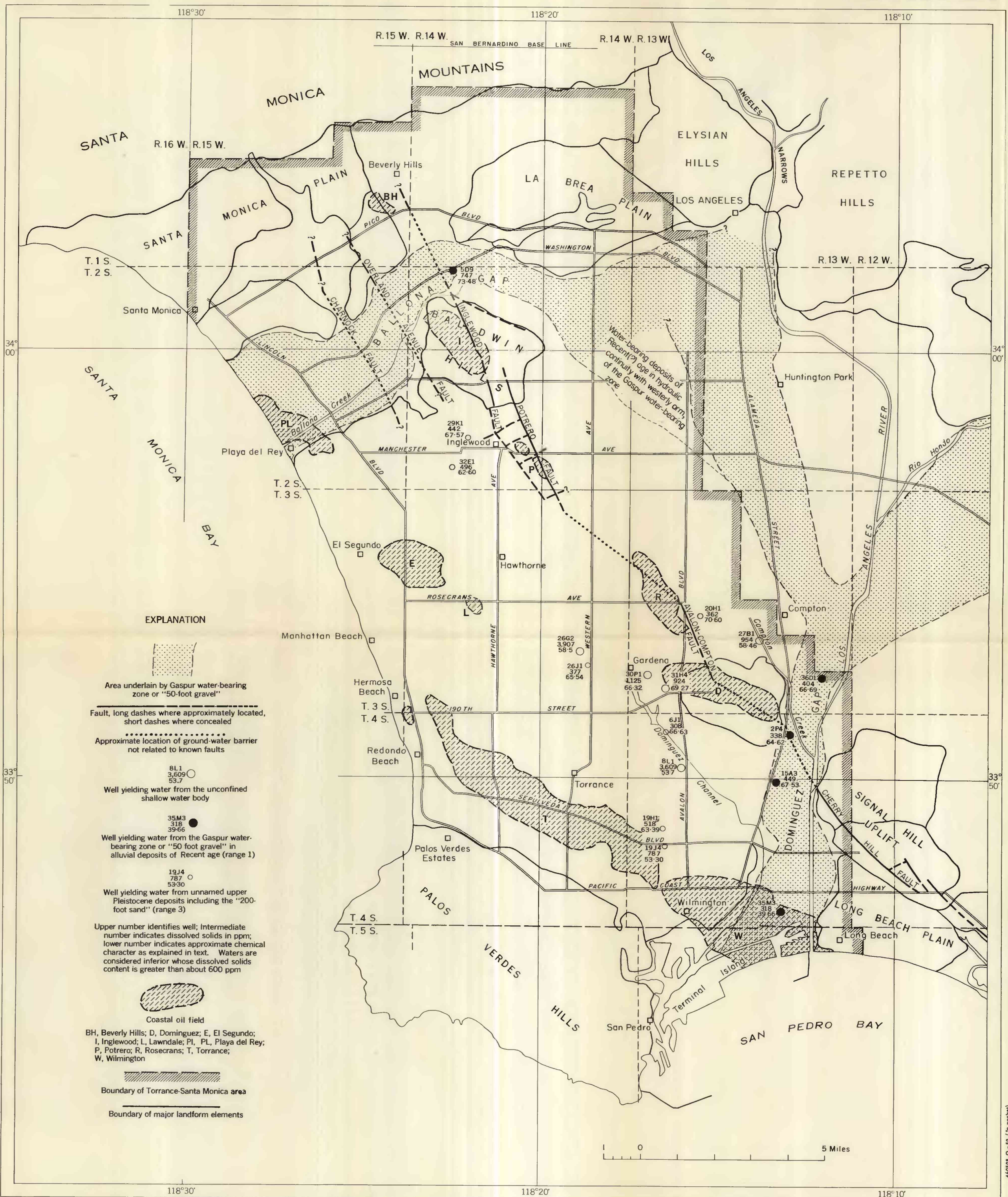
MAP OF THE TORRANCE-SANTA MONICA AREA, CALIFORNIA, SHOWING SOURCES OF REPRESENTATIVE NATIVE WATERS FROM THE SHALLOW UNCONFINED WATER BODY
