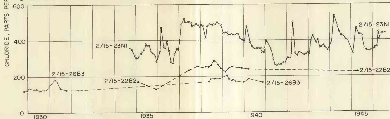
CHLORIDE CONTENT OF WATERS FROM SELECTED WELLS IN BALLONA GAP, CALIFORNIA, BETWEEN CENTINELA BOULEVARD AND THE COAST
