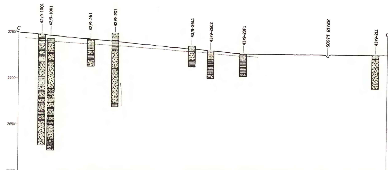
LONGITUDINAL SECTION ALONG TROUGH OF SCOTT VALLEY FROM NEAR ETNA TO FORT JONES
