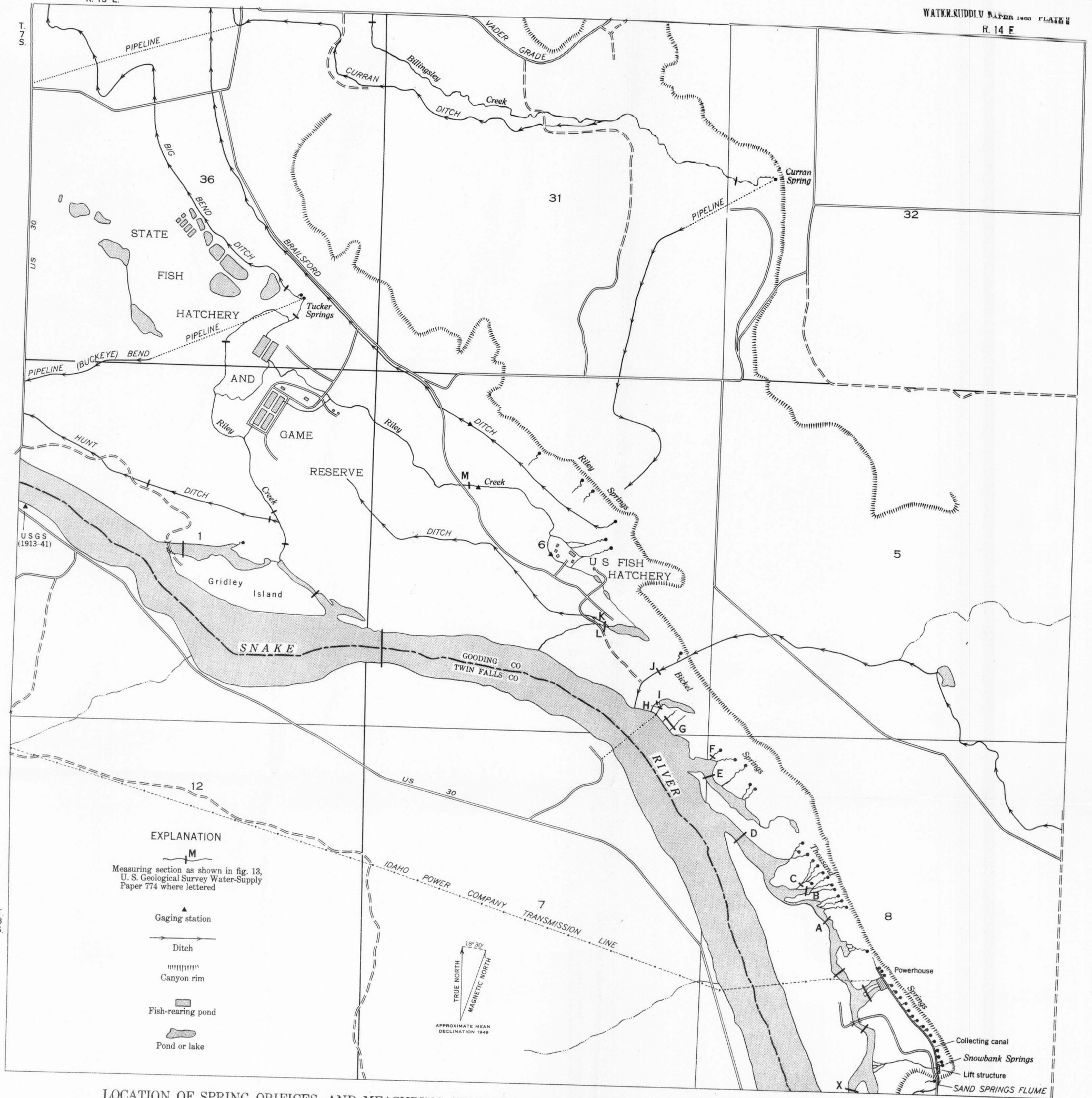
LOCATION OF SPRING ORIFICES AND MEASURING SECTIONS IN VICINITY OF THOUSAND SPRINGS AND BICKEL SPRINGS, IDAHO
