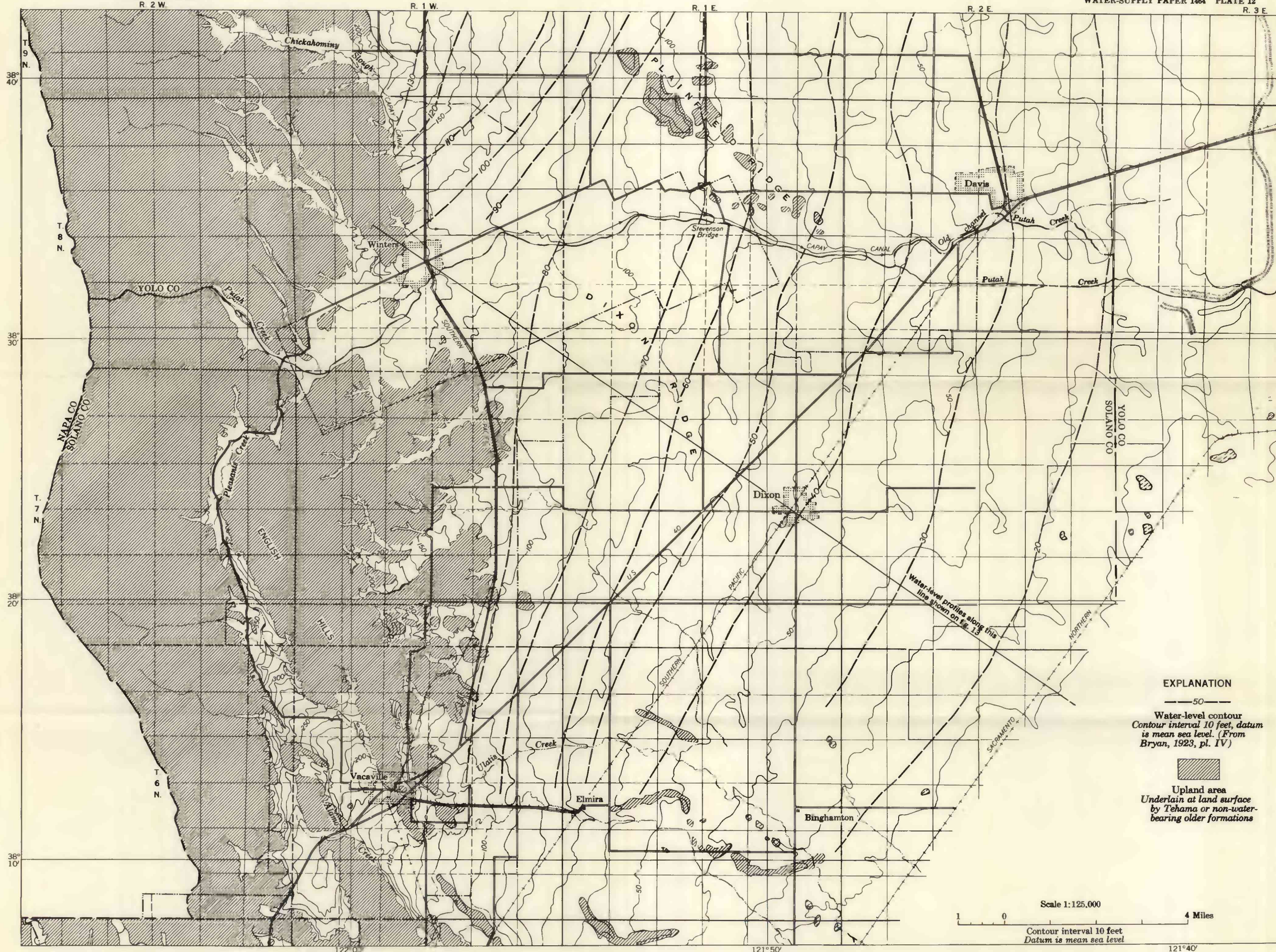
MAP OF THE PUTAH AREA, SOLANO COUNTY, CALIFORNIA, SHOWING GROUND-WATER CONTOURS, DECEMBER 1912
