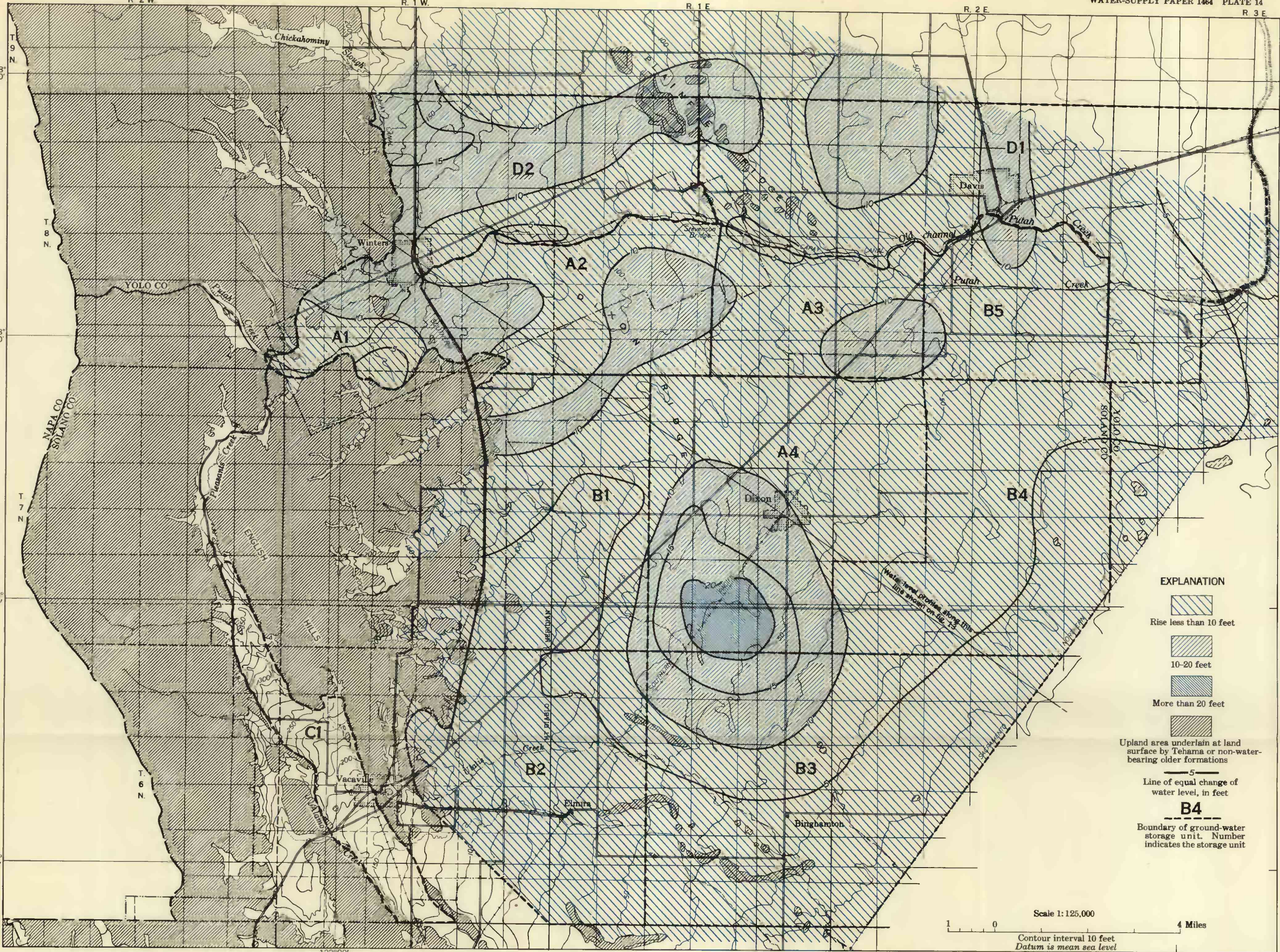
AVERAGE RISE OF THE WATER LEVEL BETWEEN APRIL 1932 AND MAY 1941
