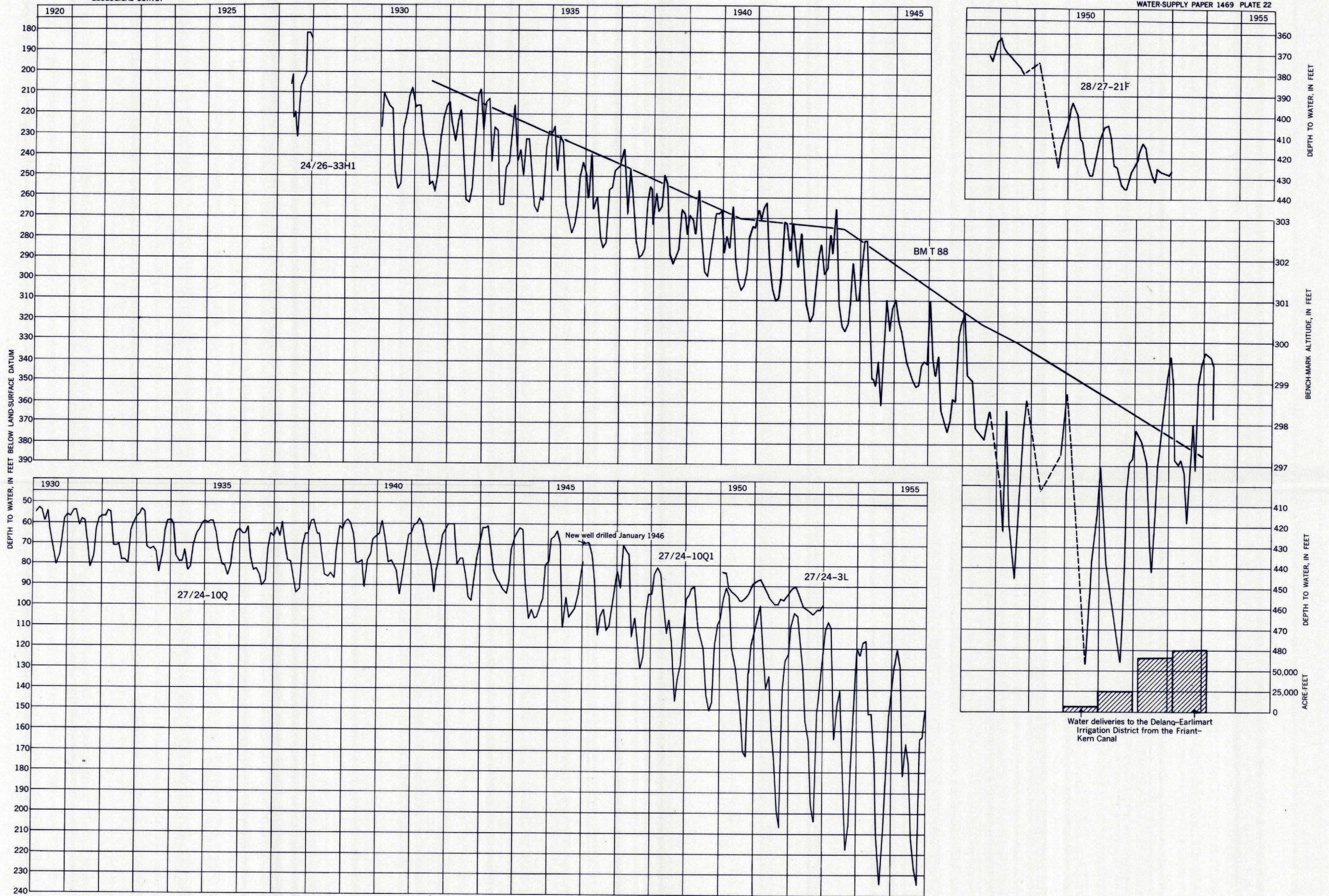
WHITE-POSO UNIT REPRESENTATIVE HYDROGRAPHS OF FIVE WELLS AND GRAPH OF BENCH MARK IN THE SOUTHEASTERN PART OF THE SAN JOAQUIN VALLEY, CALIFORNIA
