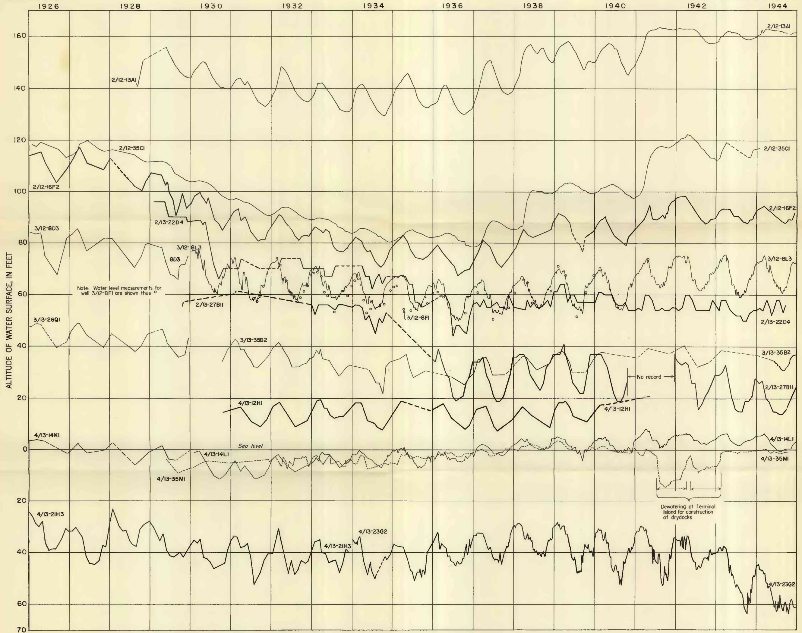
FOR WELLS IN LOS ANGELES COUNTY, CALIFORNIA REPRESENTATIVE LONG-TERM HYDROGRAPHS
