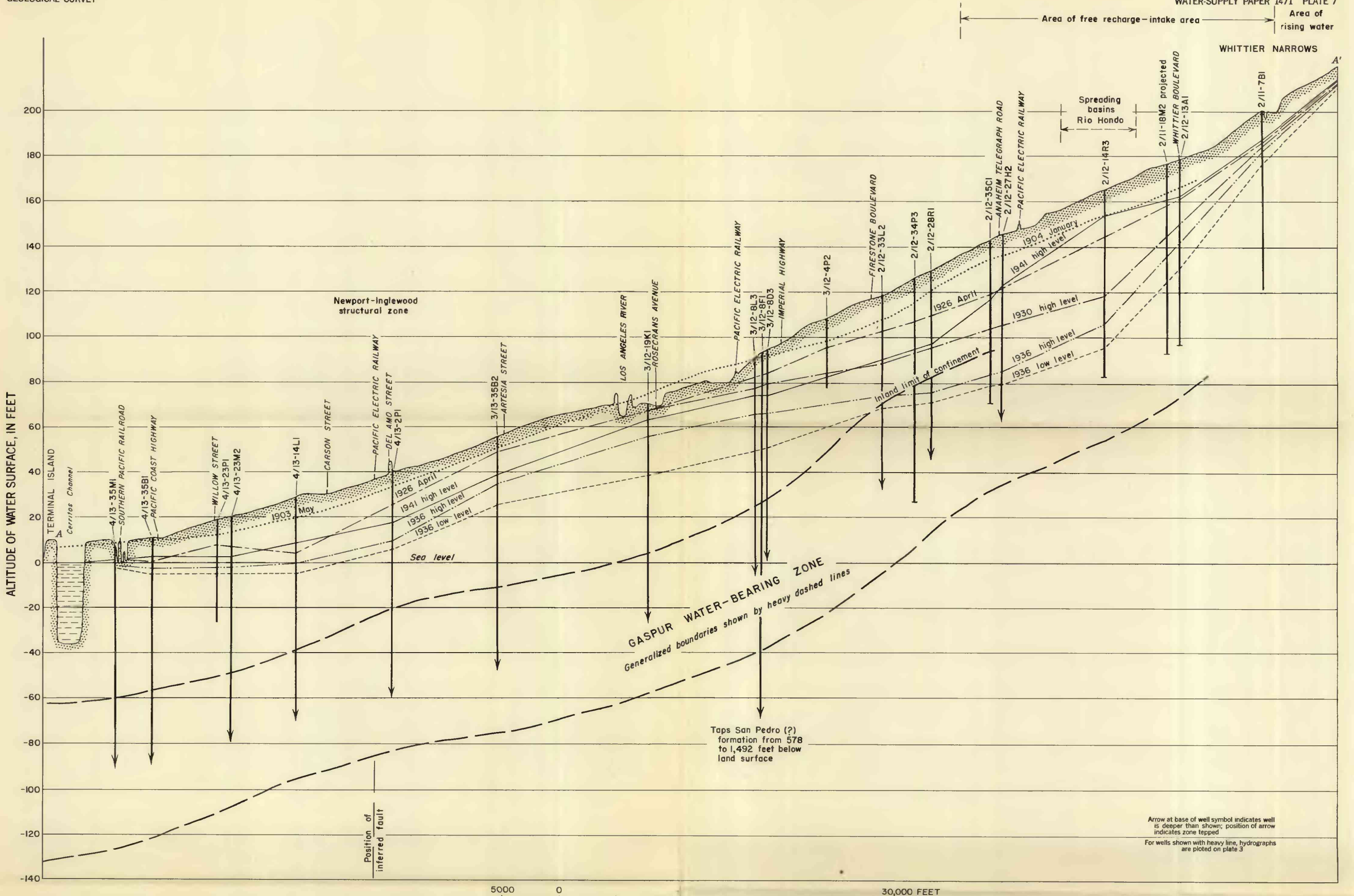
WATER-LEVEL PROFILES FOR THE GASPUR WATER-BEARING ZONE FROM TERMINAL ISLAND TO WHITTIER NARROWS, 1903-41
