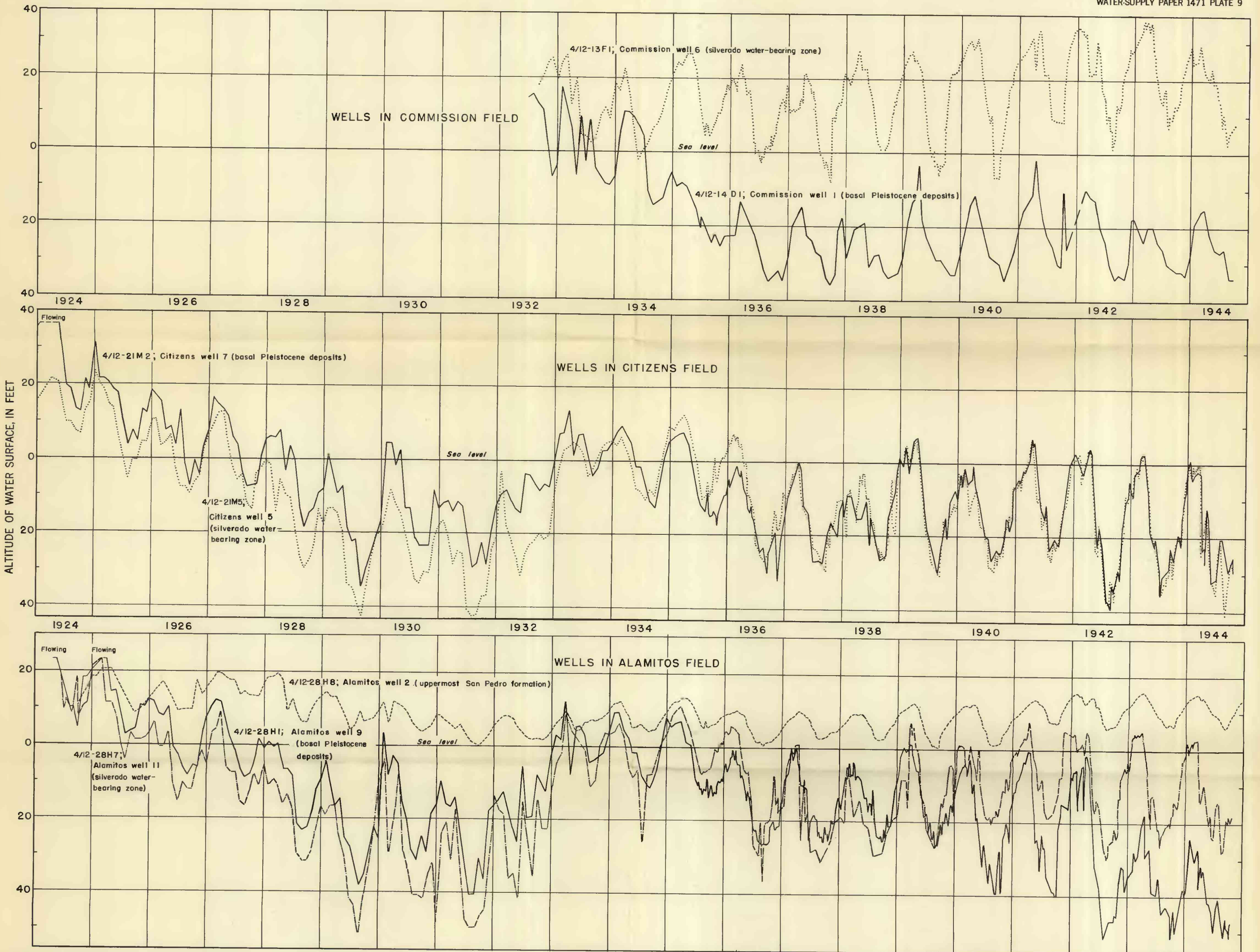
REPRESENTATIVE HYDROGRAPHS FOR WELLS IN COMMISSION, CITIZENS, AND ALAMITOS WELL FIELDS OF THE CITY OF LONG BEACH, CALIFORNIA, 1924-44
