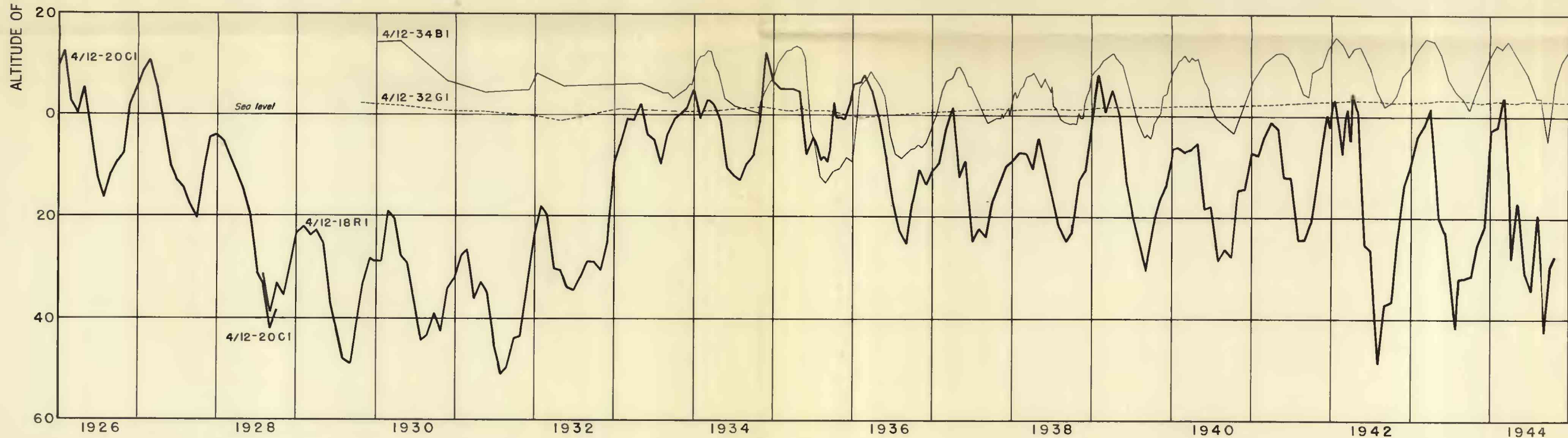
HYDROGRAPHS FOR SIX WELLS IN DOMINGUEZ GAP AND ON THE SIGNAL HILL UPLIFT TAPPING DEPOSITS OF PLEISTOCENE AGE, 1926-44
