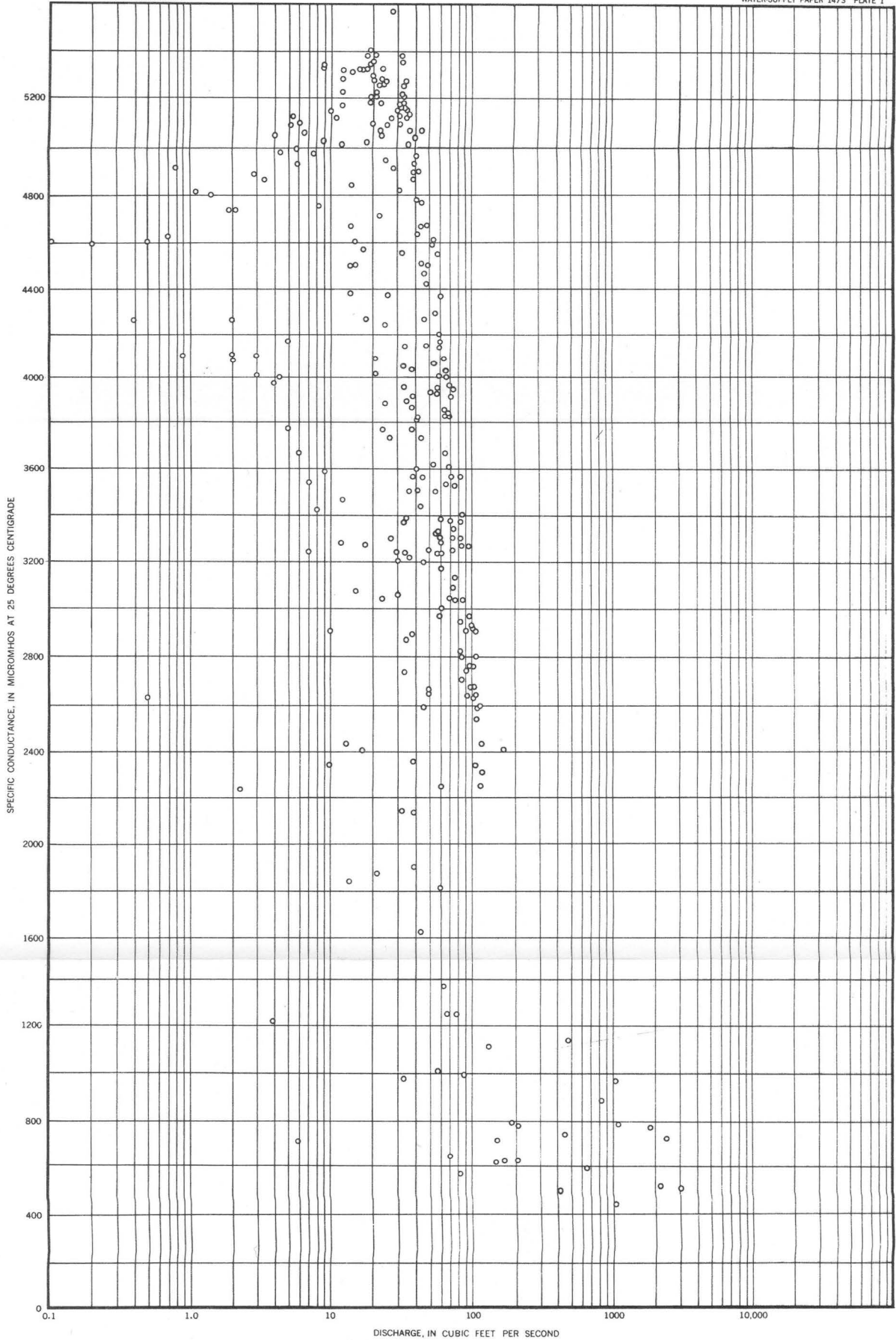
SPECIFIC CONDUCTANCE OF DAILY SAMPLES AND MEAN DAILY DISCHARGE, GILA RIVER AT BYLAS, ARIZONA, OCTOBER 1, 1943, TO SEPTEMBER 30, 1944
