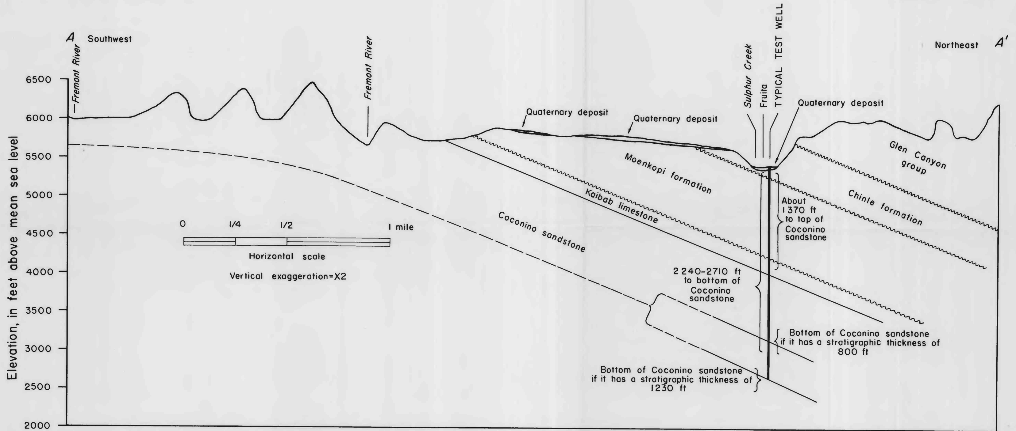
GEOLOGIC SECTION A-A' SHOWING ESTIMATED DEPTH OF A TYPICAL WATER-TEST WELL IN THE VICINITY OF FRUITA, UTAH
