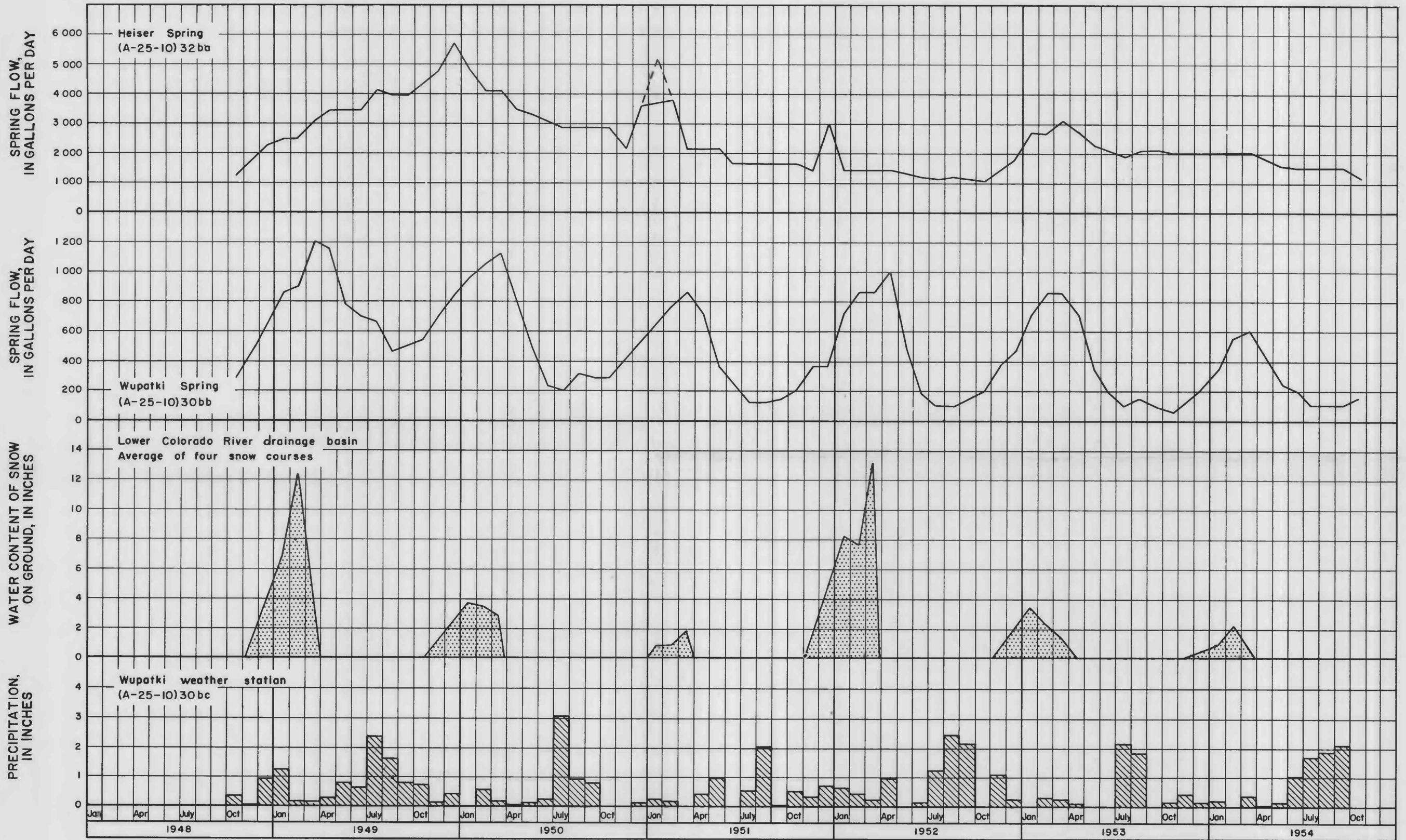
DISCHARGE OF HEISER AND WUPATKI SPRINGS COMPARED WITH WATER CONTENT OF SNOW ON GROUND AND PRECIPITATION, WUPATKI NATIONAL MONUMENT, COCONINO COUNTY, ARIZONA
