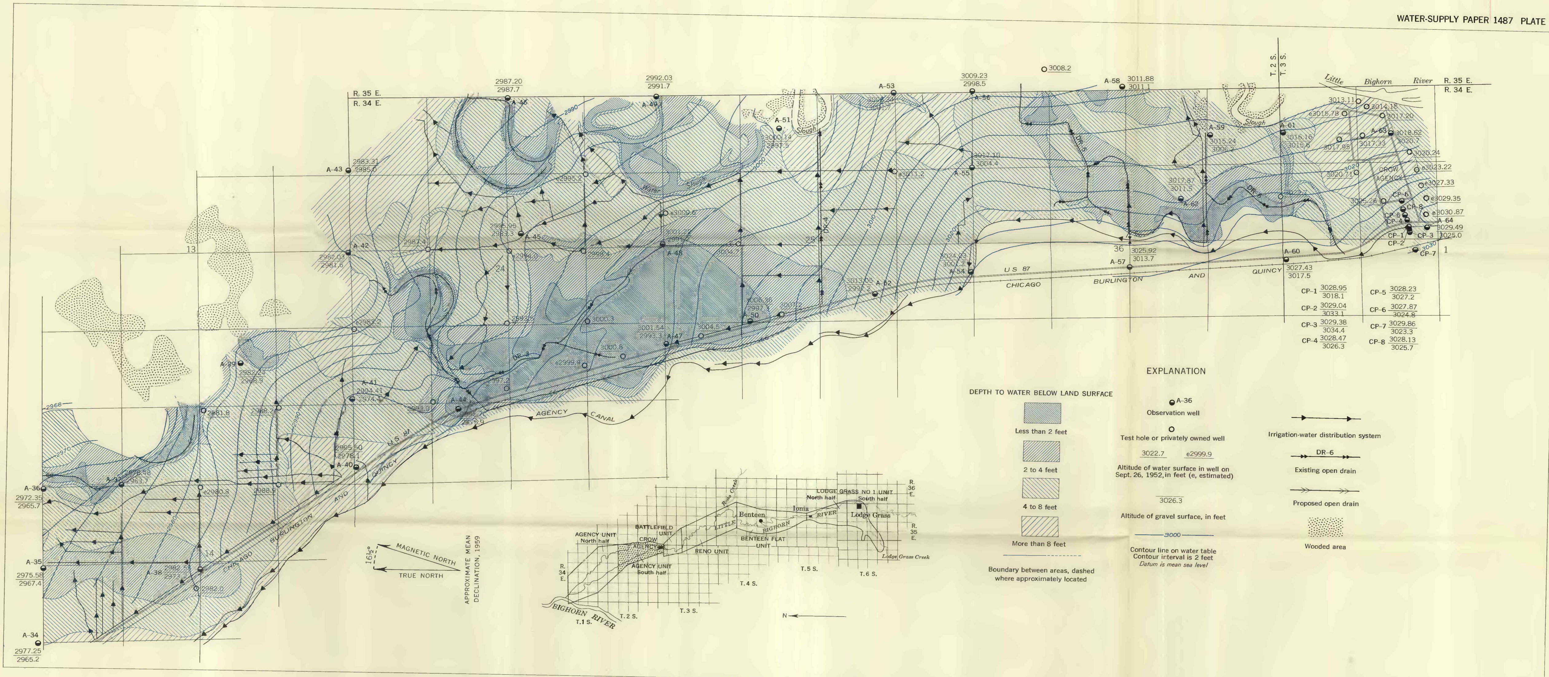
MAP OF THE SOUTH HALF OF THE AGENCY UNIT, BIG HORN COUNTY, MONTANA, SHOWING DEPTH TO WATER, CONTOUR OF THE WATER TABLE, ALTITUDE OF THE GRAVEL SURFACE, AND LOCATIONS OF EXISTING AND PROPOSED DRAINS
